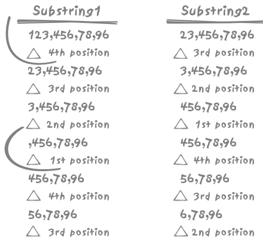
FIGURE 11-4. Splitting-up a comma separated list
