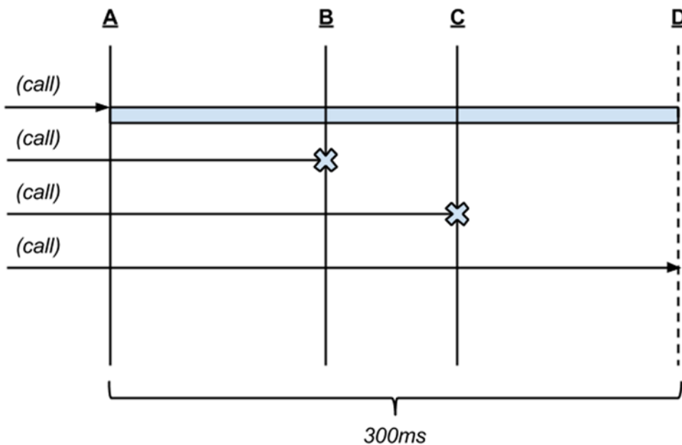
Figure 16-2. A throttled function invoked multiple times
