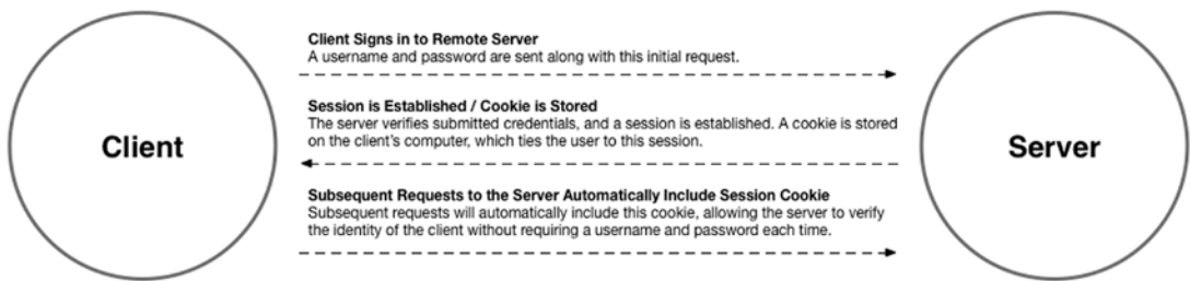
Figure 9-10. Cookie-based authentication
