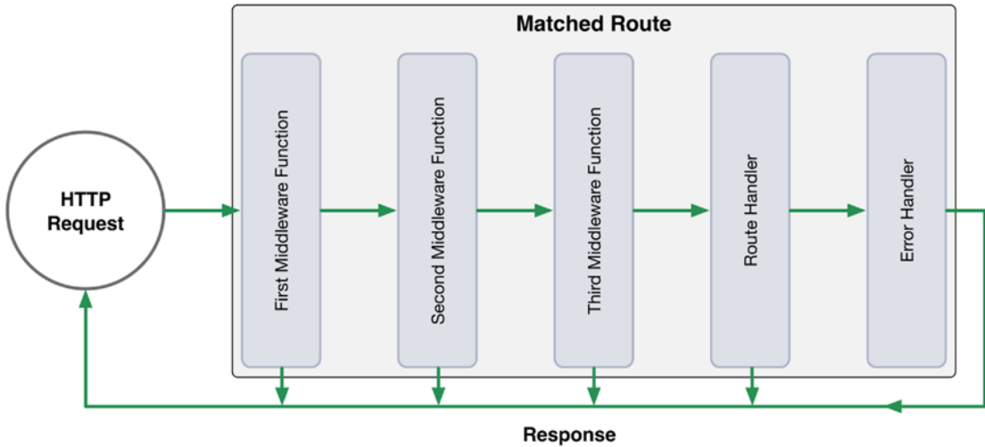
Figure 9-2. Series of Express middleware calls
