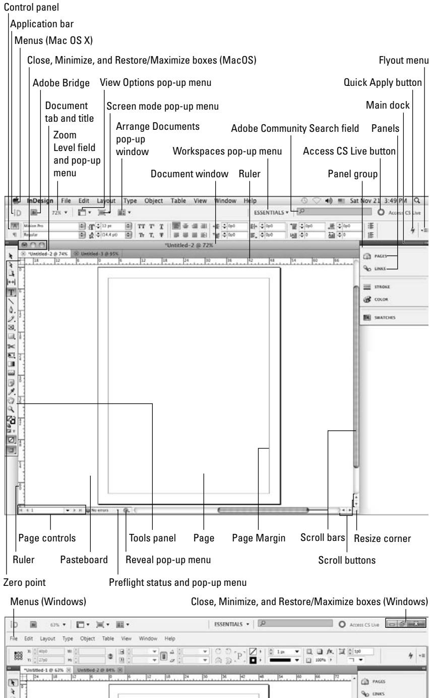
Figure 1-1: The document window is where you work on documents. Bottom: The Windows 7 version differs in its Close, Minimize, and Restore/Maximize controls.
