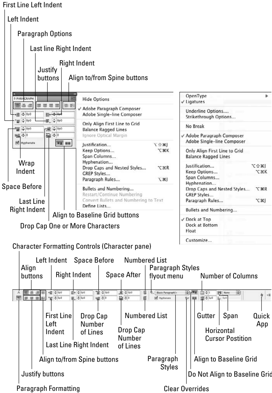
Figure 14-1: Top: The full Paragraph panel. Bottom: The Control panel's Paragraph (¶) pane.
