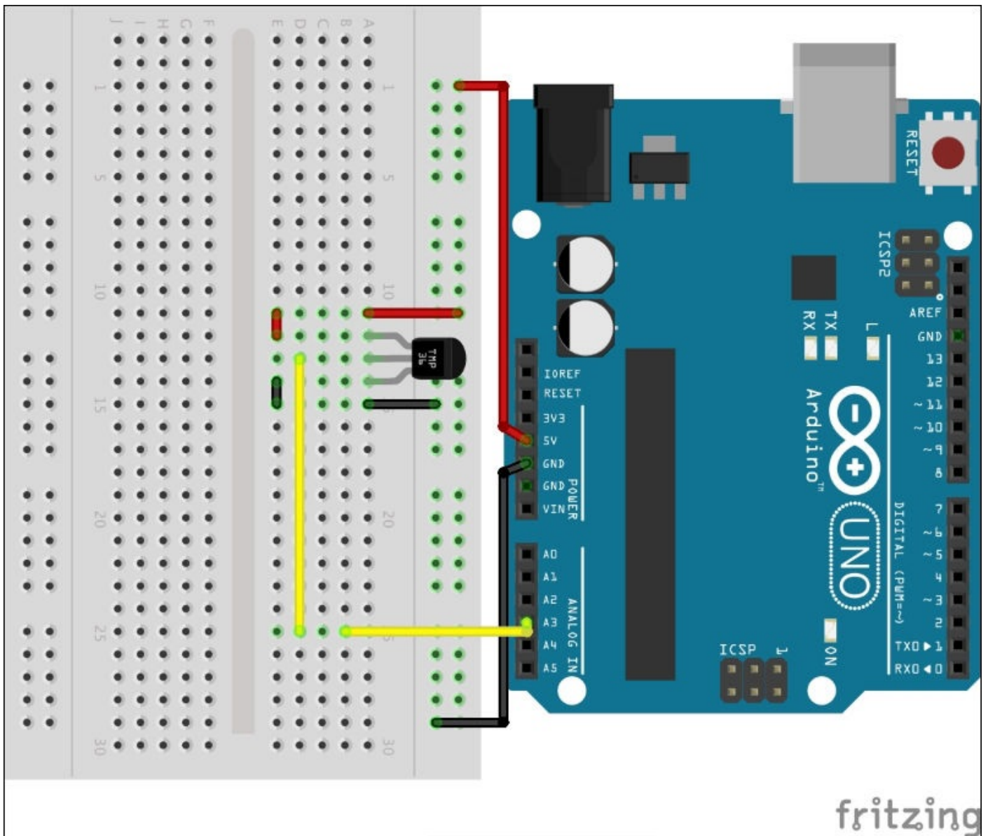
Our design - designed using Fritzing
