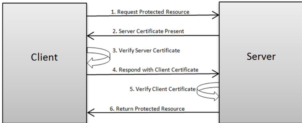
Figure 8-4. Certificate-based security flow
