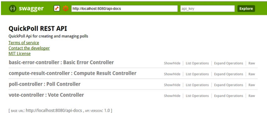
Figure 6-3. Updated QuickPoll Swagger UI
