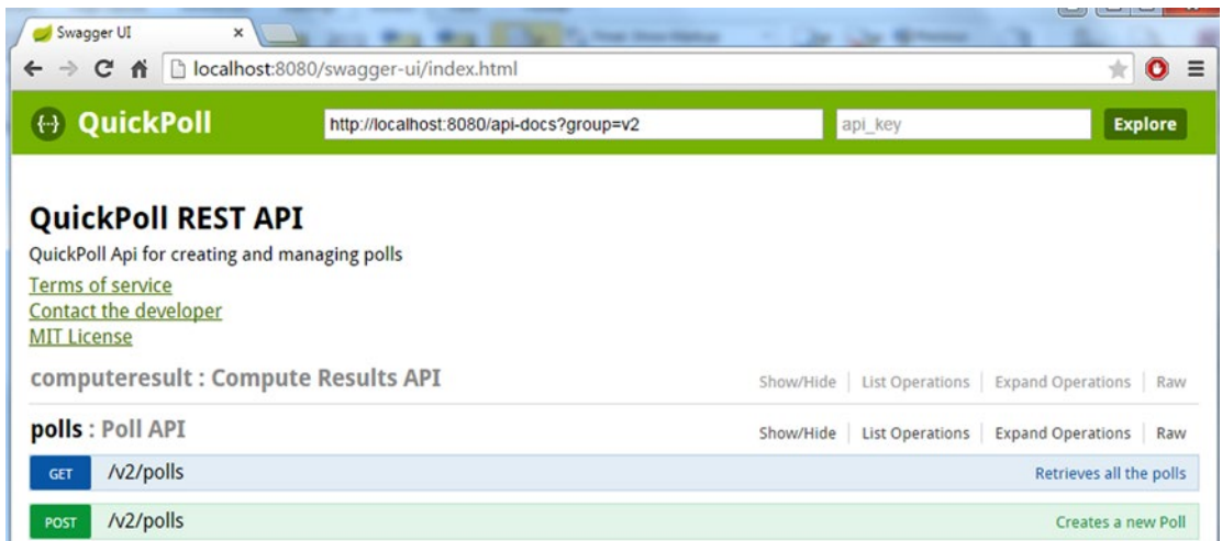
Figure 7-1. Swagger UI for QuickPoll 2.0 version
