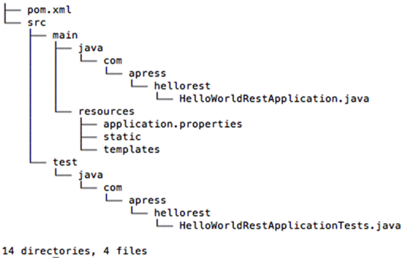
Figure 3-3. hello-rest application contents
