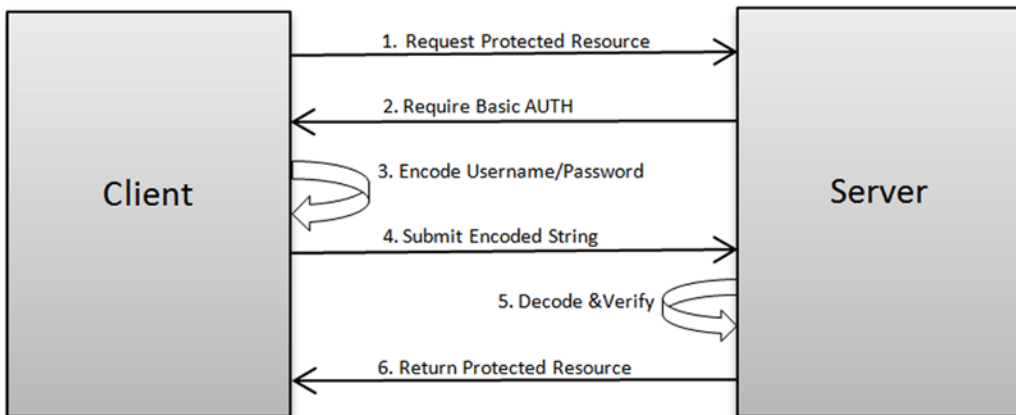
Figure 8-2. HTTP Basic authentication flow
