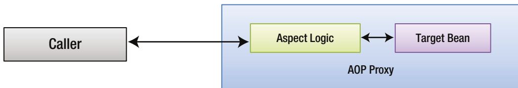
Figure 2-2. Spring AOP Proxy
