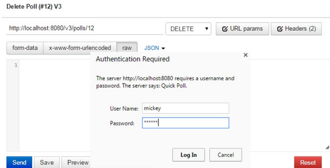
Figure 8-8. Deleting poll with unauthorized users
