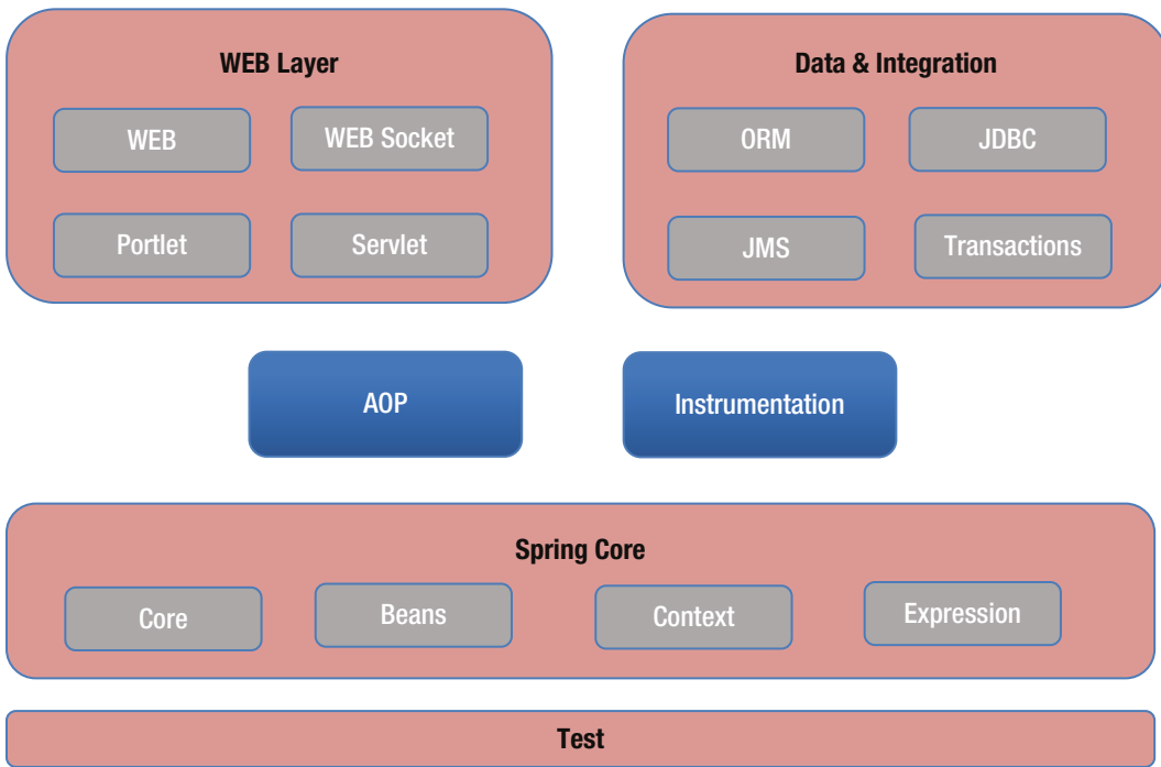
Figure 2-1. Spring Framework modules
