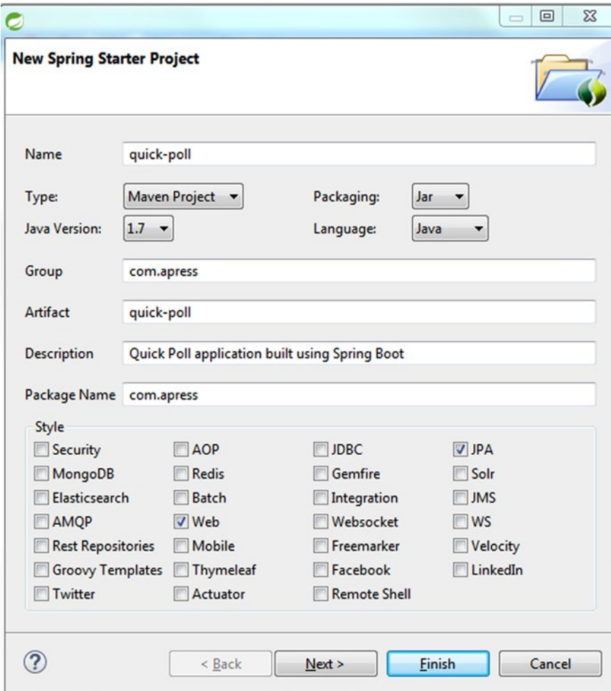
Figure 4-4. QuickPoll project configuration
