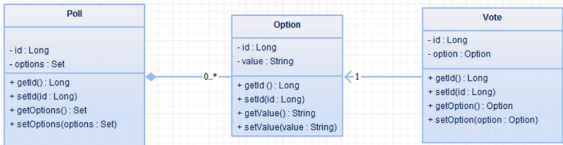
Figure 4-5. QuickPoll domain objects
