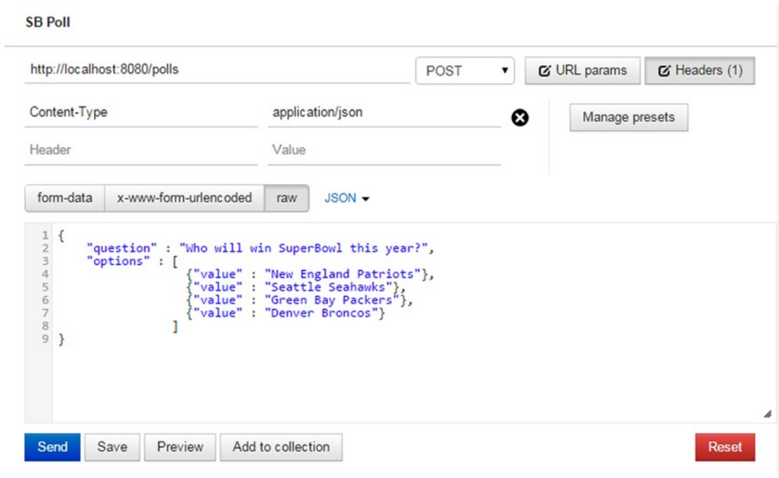
Figure 4-7. Create Poll Postman example
