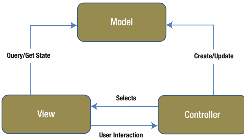
Figure 2-3. Model View Controller interaction
