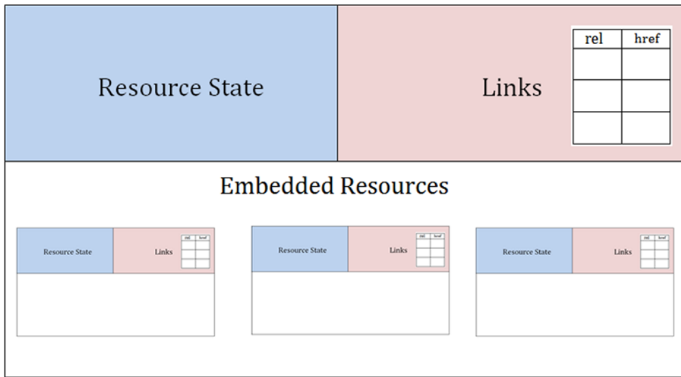
Figure 10-1. HAL resource structure
