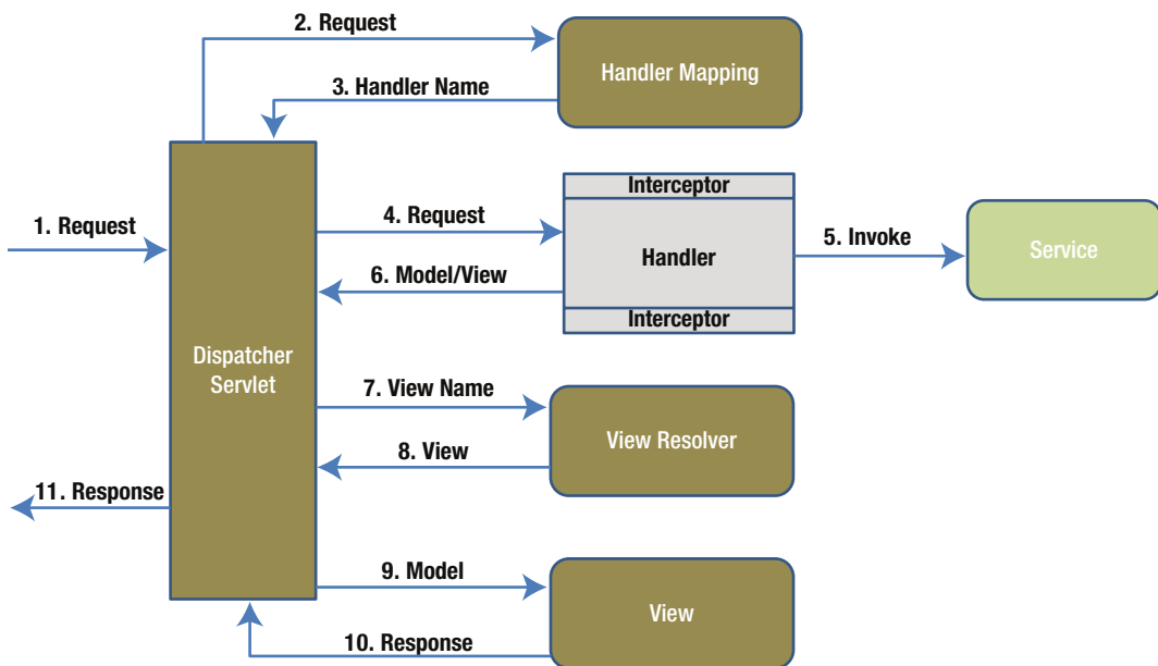
Figure 2-4. Spring Web MVC's architecture
