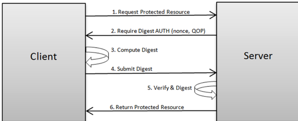
Figure 8-3. Digest authentication flow
