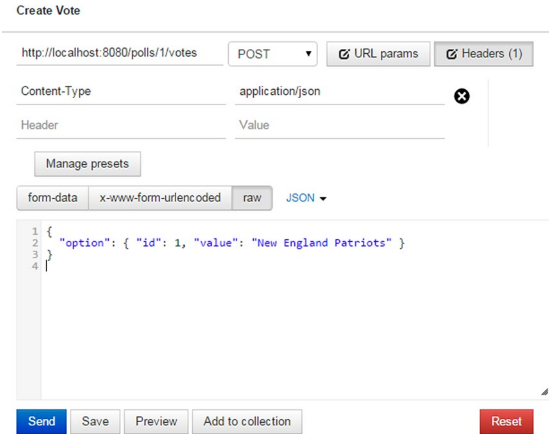
Figure 4-9. Cast a new vote
