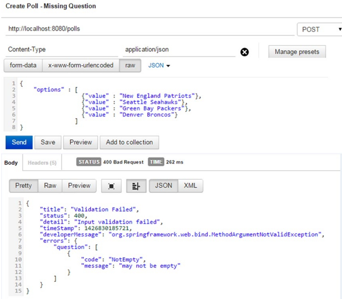
Figure 5-9. Validation error response
