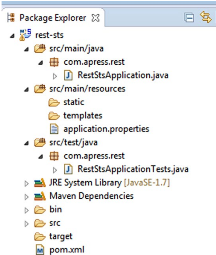
Figure 3-8. STS Spring starter project resources
