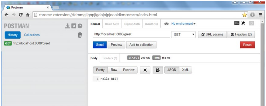
Figure 3-11. Postman browser extension
