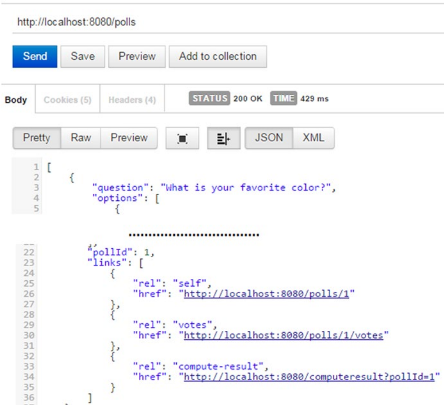
Figure 10-2. Postman response with links
