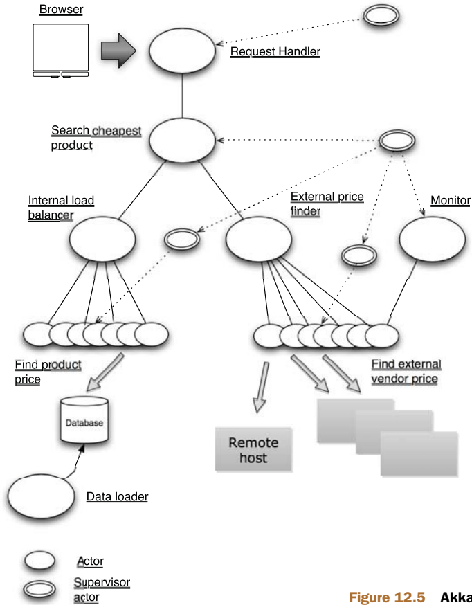
Figure 12.5 Akkaoogle architecture
