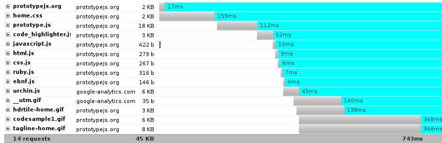
Figure 9.1: The two-request limit in action at http://prototypejs.org
