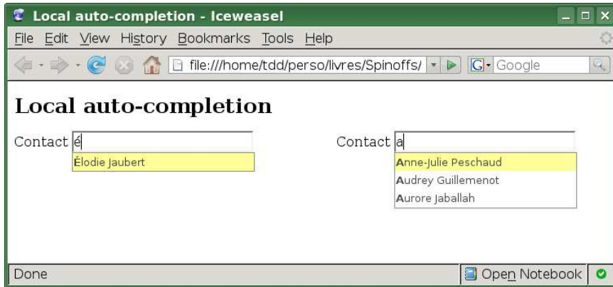
Figure 16.2: Same views, with “standard” styling
