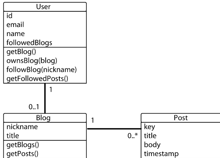
Figure 30—The blog model in UML
