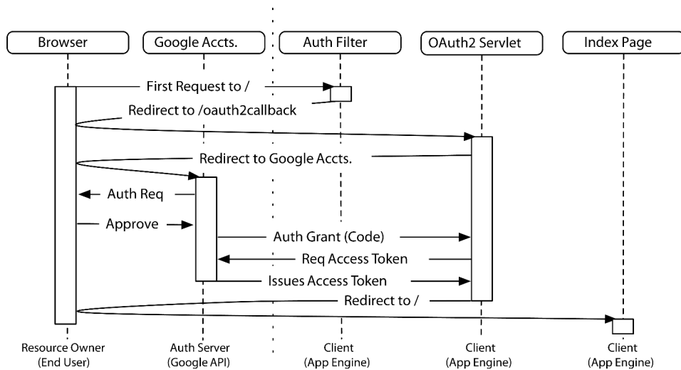
Figure 11—OAuth 2.0 protocol flow
