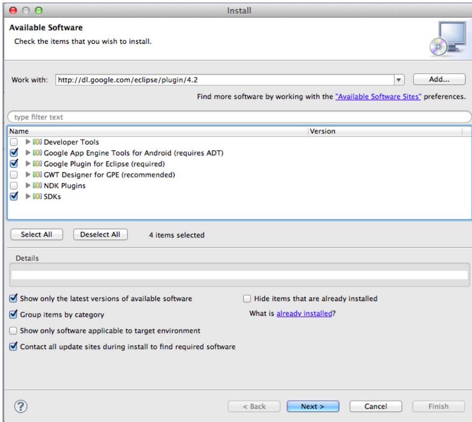
Figure 4—Adding the GAE plug-ins to Eclipse
