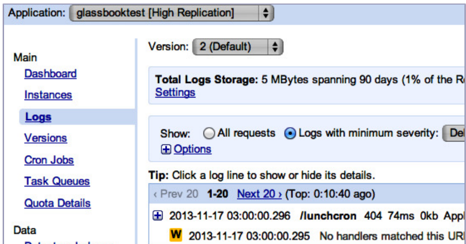
Figure 23—Google App Engine logs
