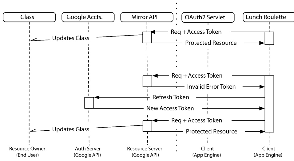
Figure 12—Using an access token to issue Mirror API requests
