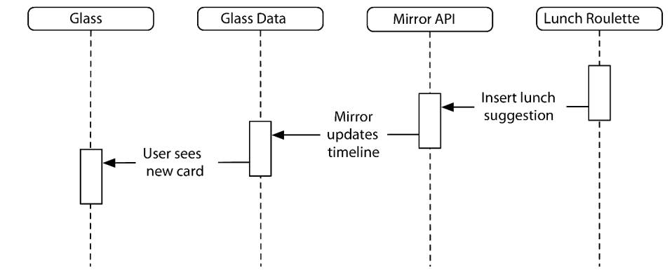
Figure 13—Flow of Glassware to Glass
