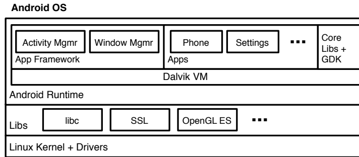
Figure 35—Android OS Layers
