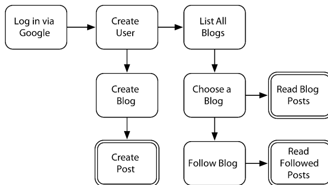
Figure 32—Blog actions flow chart
