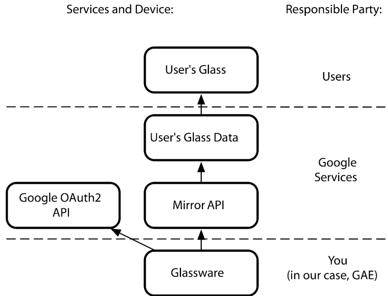
Figure 2—The actors in creating Glassware using the Mirror API
