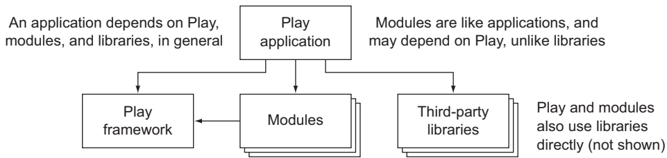
Figure 3.16 Play application dependencies on libraries, modules, and the framework itself
