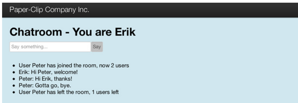
Figure 10.8 WebSockets chatroom
