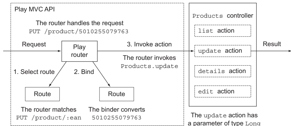
Figure 4.5 Routing requests: binding parameters and invoking controller actions
