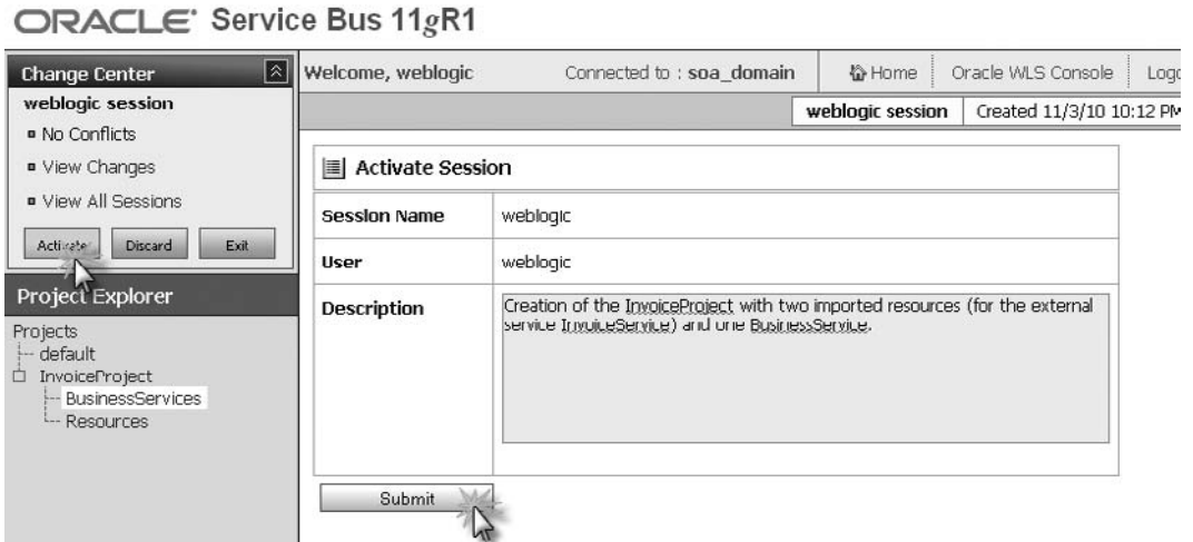
FIGURE 13-8. Activating the changes in the current session through the Change Center
