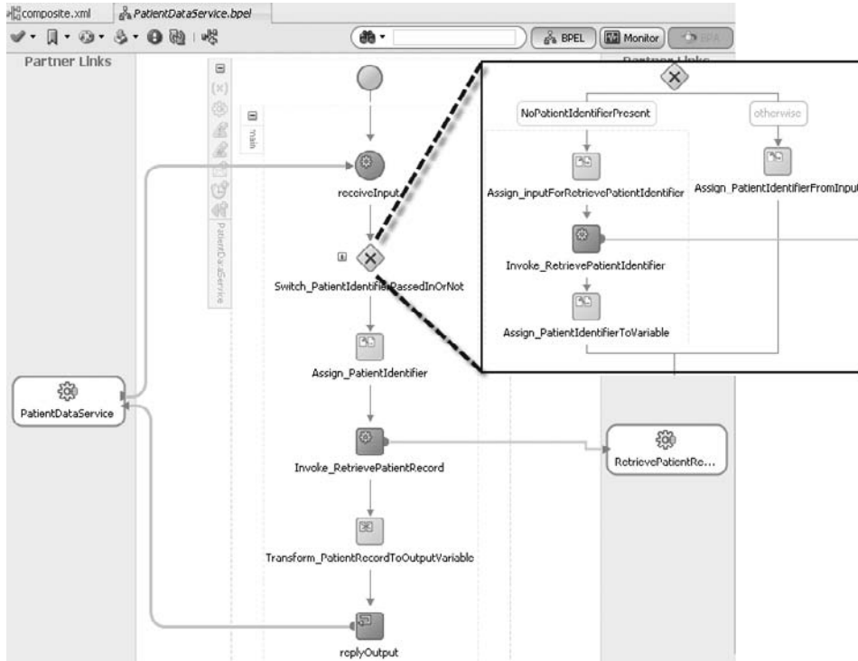
FIGURE 5-22. The complete PatientDataService BPEL process
