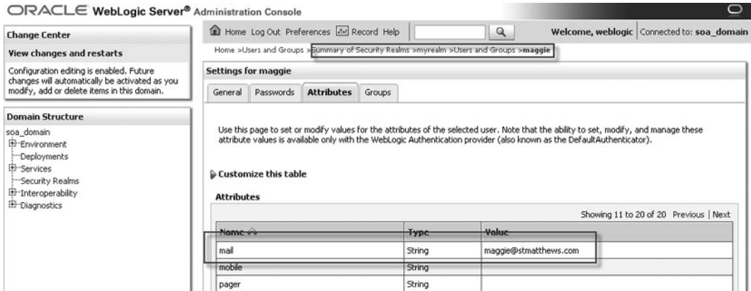
FIGURE 10-15. Set mail attribute for user Maggie in the WLS Console
