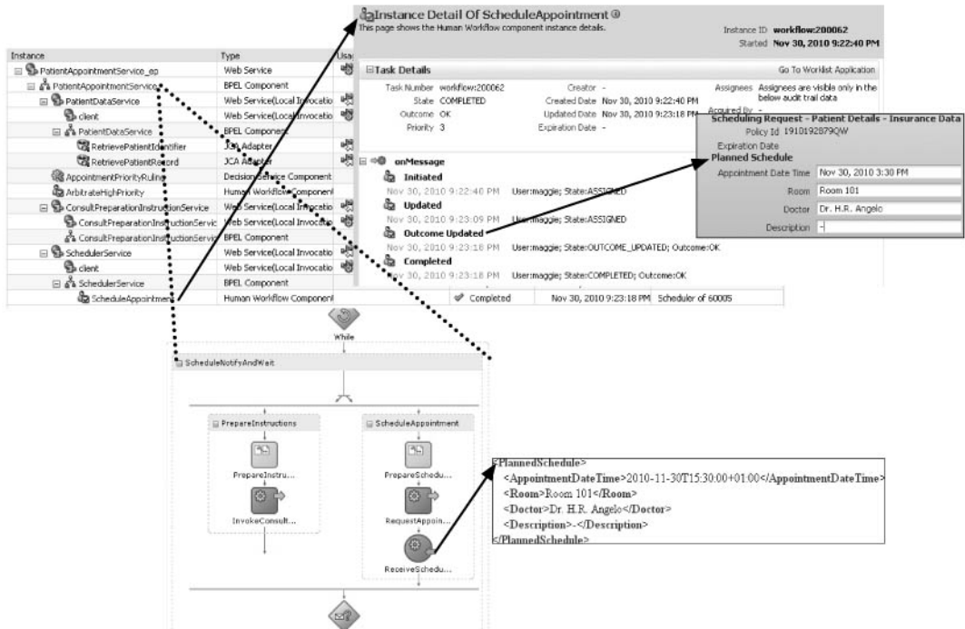
FIGURE 10-26. Message flow trace showing the ScheduleAppointment task's results being passed back
