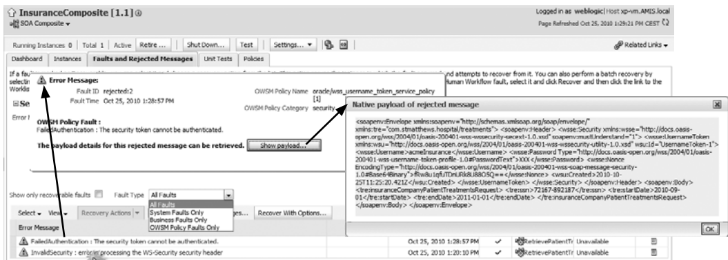
FIGURE 15-16. Inspecting OWSM policy faults
