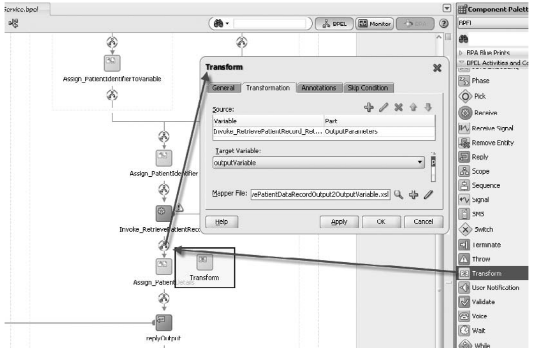
FIGURE 5-19. Adding a Transform activity to the BPEL process to populate the outputVariable with the patient data record
