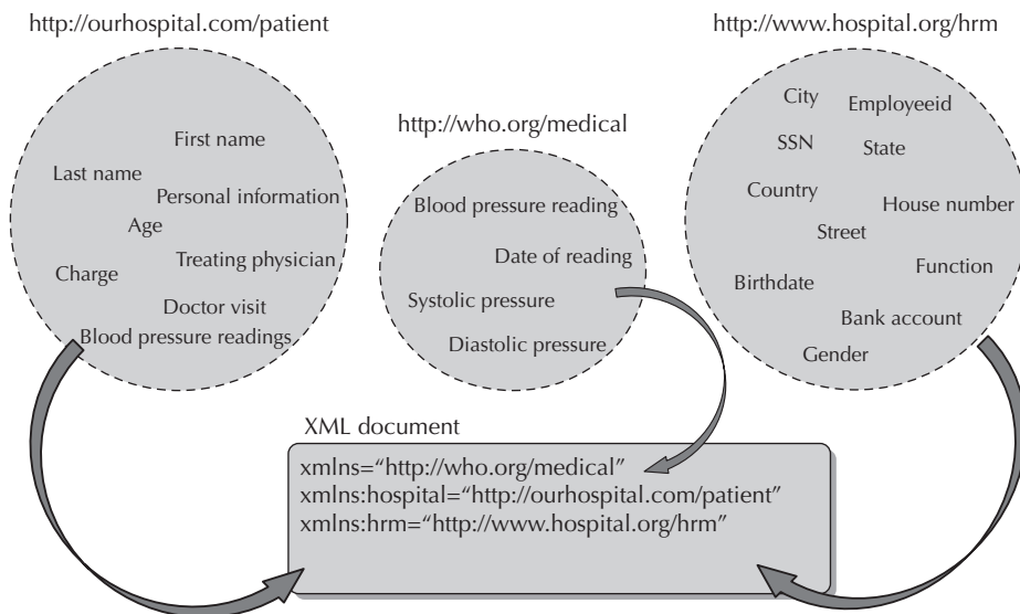
FIGURE 4-1. Namespaces for elements in different domains
