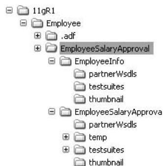
FIGURE A-7. The result of the migration; the two BPEL projects are under the project folder.
