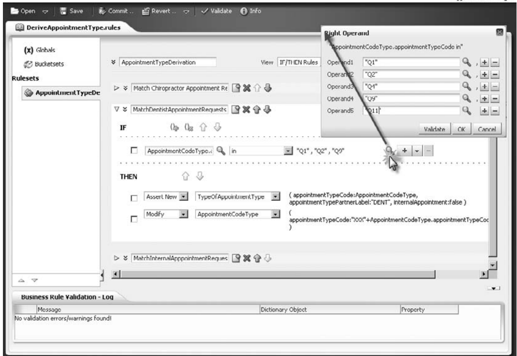
FIGURE 8-14. Editing the business rule for matching dental appointment requests—adding the two new codes Q9 and Q11 that must be supported
