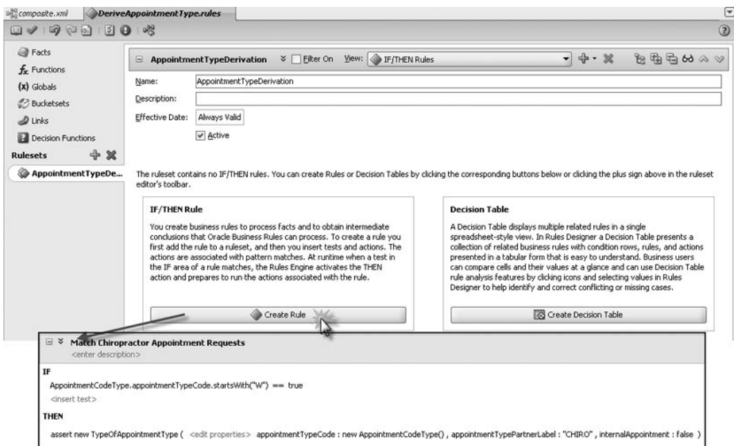
FIGURE 8-2. Add the first IF/THEN rule to the rule set
