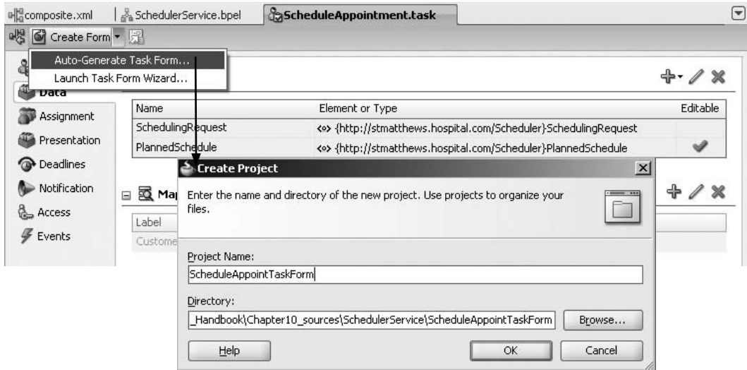
FIGURE 10-22. Generating the task form for ScheduleAppointment
