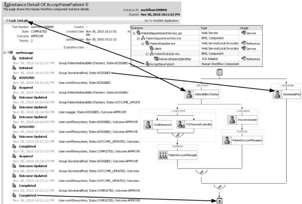
FIGURE 10-32. An appointment request for a new patient has started the accept new patient task
