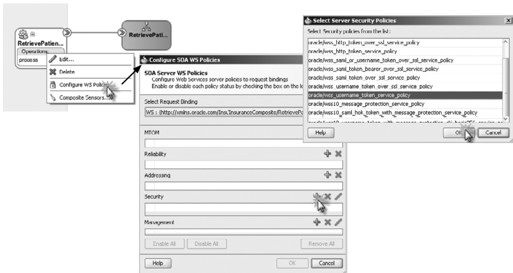
FIGURE 15-24. Adding policies to a SOA composite using JDeveloper
