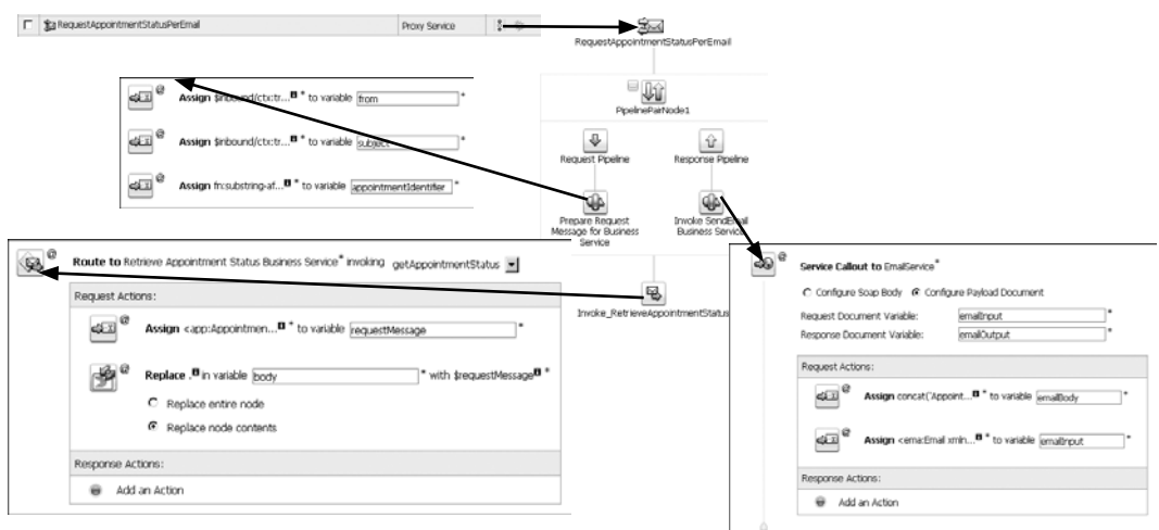
FIGURE 13-25. Configuring the message flow for the proxy service with the service callout to the EmailService
