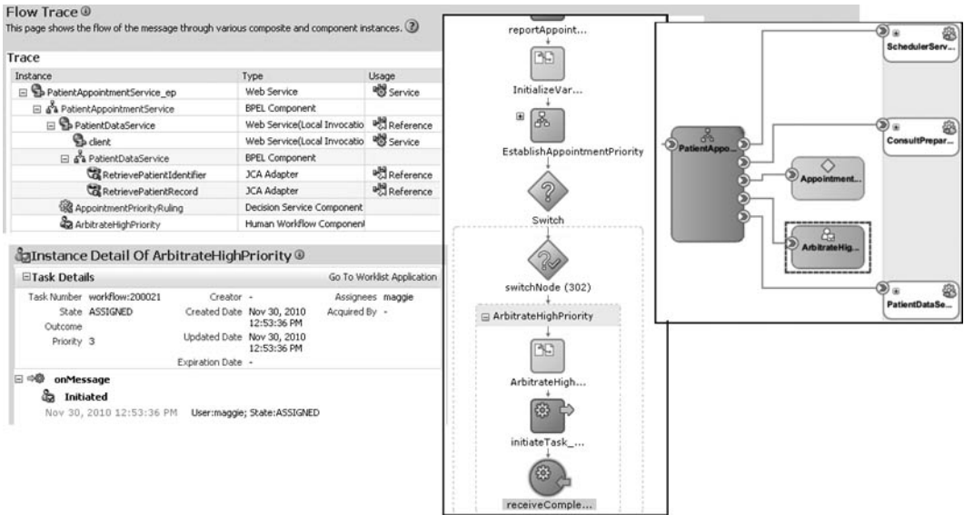
FIGURE 10-12. The message flow trace for the High priority appointment request—waiting for Maggie to act
