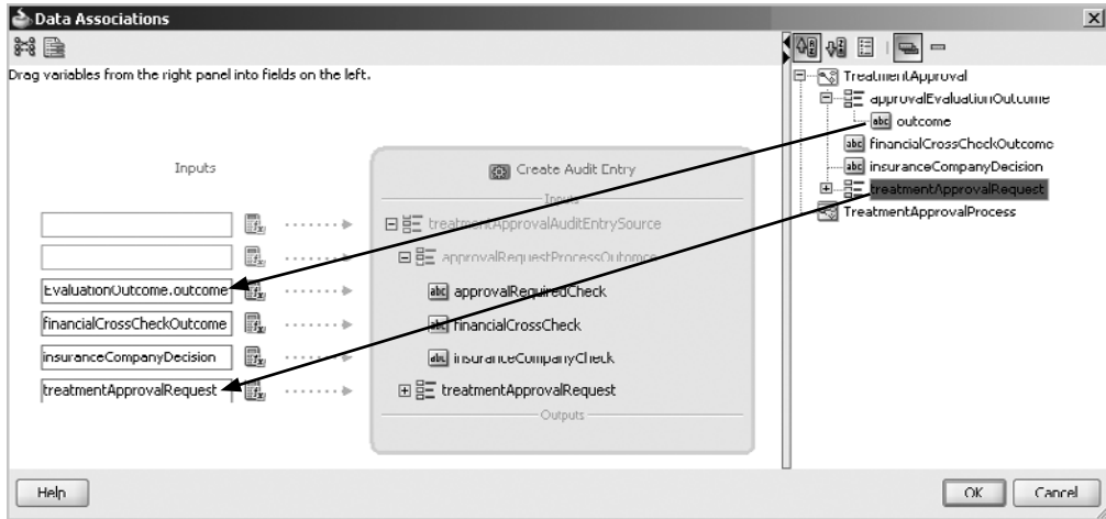
FIGURE 11-20. Creating data associations for the mapping of the service task Create Audit Entry
