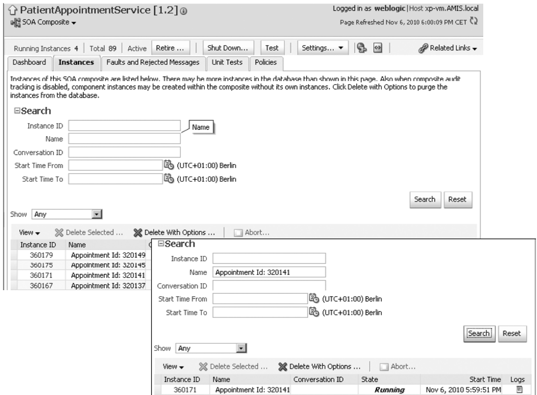
FIGURE 16-7. Instances for which the name has been set are easier to identify and find.
