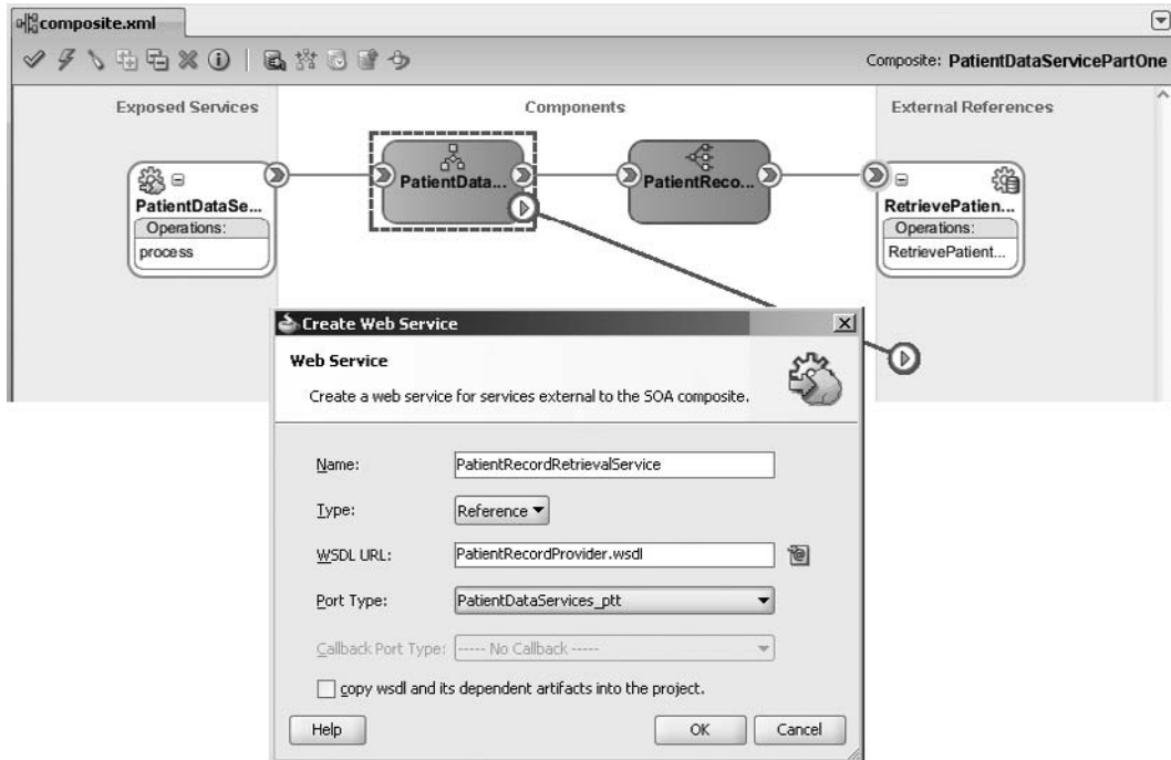
FIGURE 14-6. Breaking up the PatientDataService composite. Part One will lose the PatientRecordProvider Mediator ; the reference that the Mediator currently satisfies needs to be exposed at the composite level.
