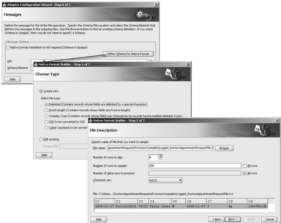
FIGURE 7-3. Using the Native Format Builder to create an XSD for the CSV file format
