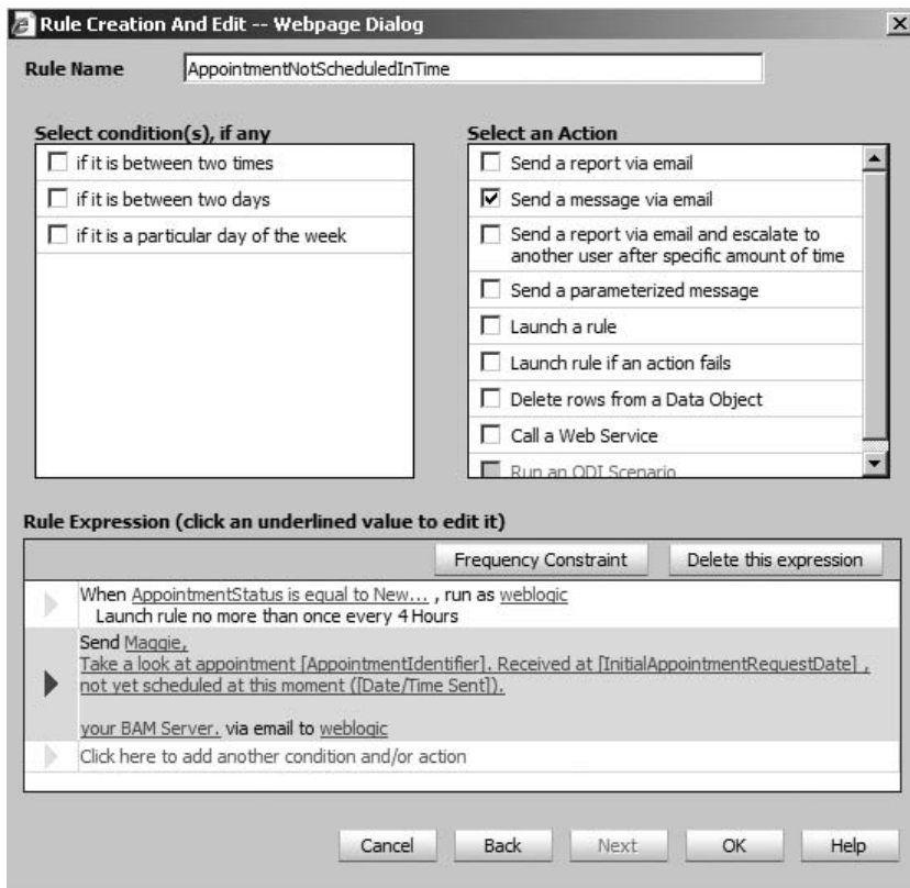
FIGURE 19-34. Specifying the action for the non-event alert for not scheduling the appointment
