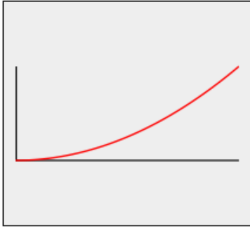
Quad.easeIn
