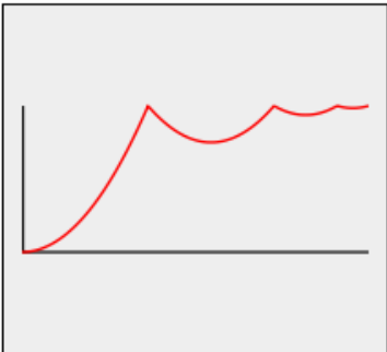
Bounce.easeOut
