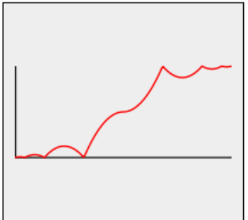
Bounce.easeInOut
