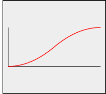
Quad.easeInOut
