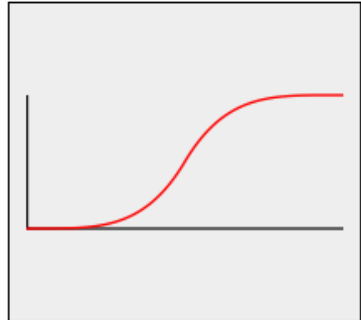
Quart.easeInOut
