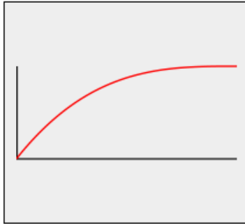
Cubic.easeOut
