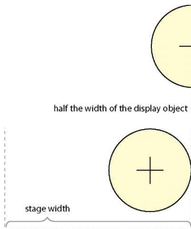
Figure 7-9. When testing for boundary collisions on display objects with a center registration point (top) and when subtracting half the width of the object from the stage dimensions (bottom).
