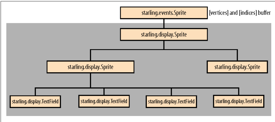
Figure 23. When flattened, children drawn in one draw call (one index/vertex buffer)
