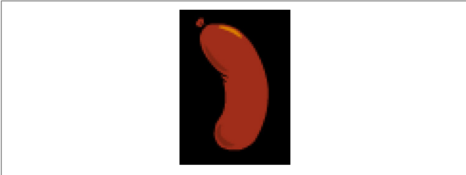
Figure 18. TextureSmoothing.NONE
