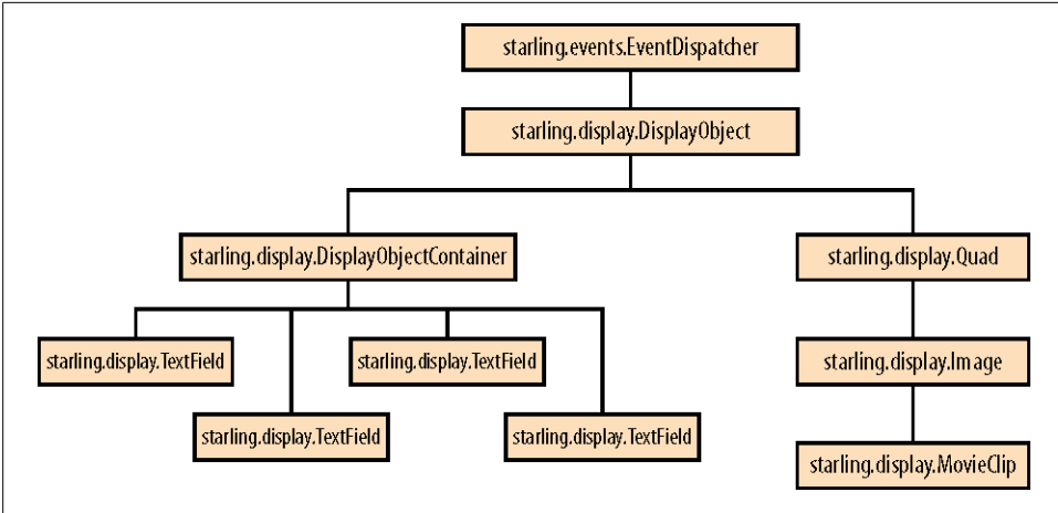
Figure 2. DisplayObject inheritance
