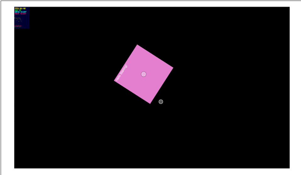
Figure 14. Multi-touch simulation
