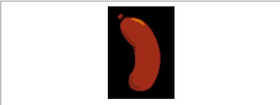
Figure 16. TextureSmoothing.BILINEAR
