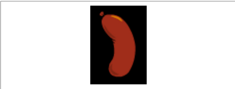
Figure 17. TextureSmoothing.TRILINEAR
