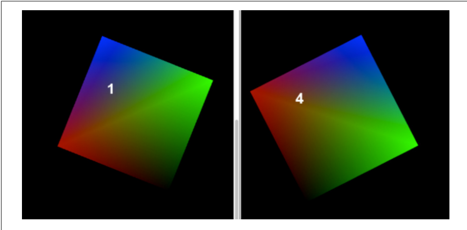
Figure 9. Anti-aliasing differences
