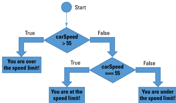
Figure 9-4: If-else with an else if statement.
