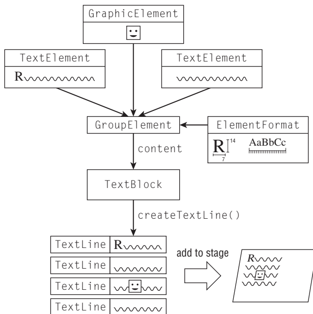
Flash Text Engine architecture
