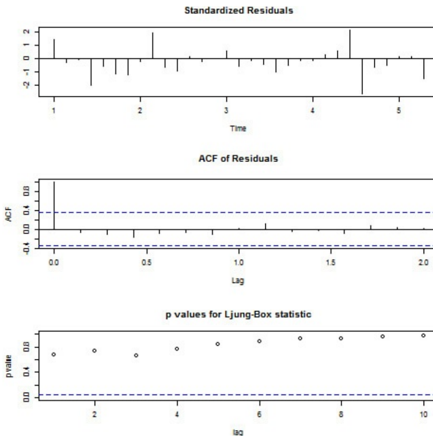
FIGURE 17.23 Diagnostic plots from seasonal ARIMA (1, 0, 1) fit
