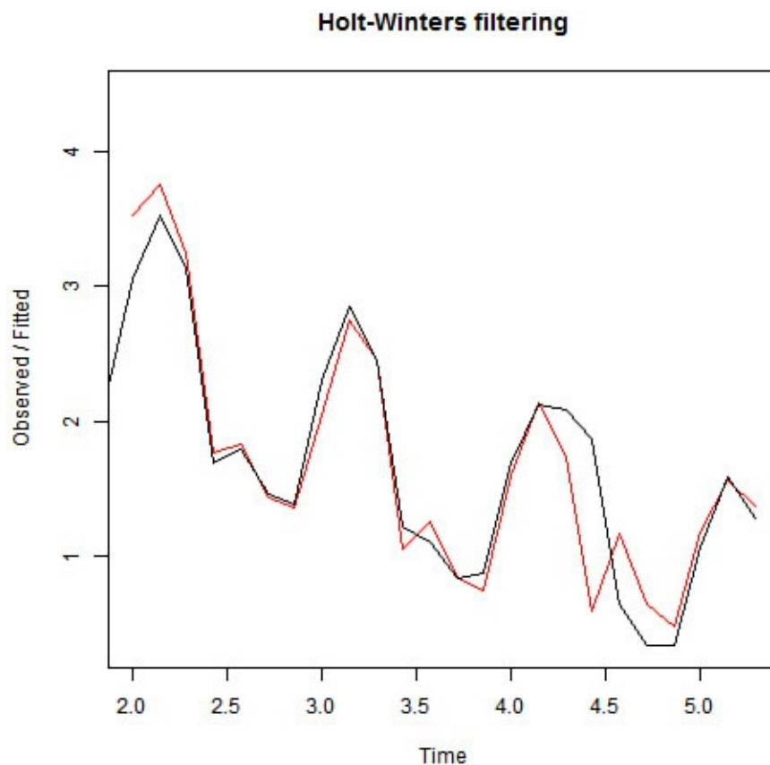
FIGURE 17.19 Holt-Winters filtering of the logged daily box office takings for Avengers: Age of Ultron
