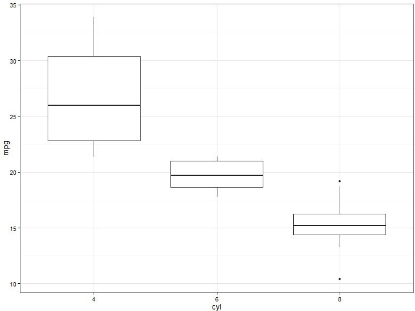
FIGURE 14.2 Generating boxplots
