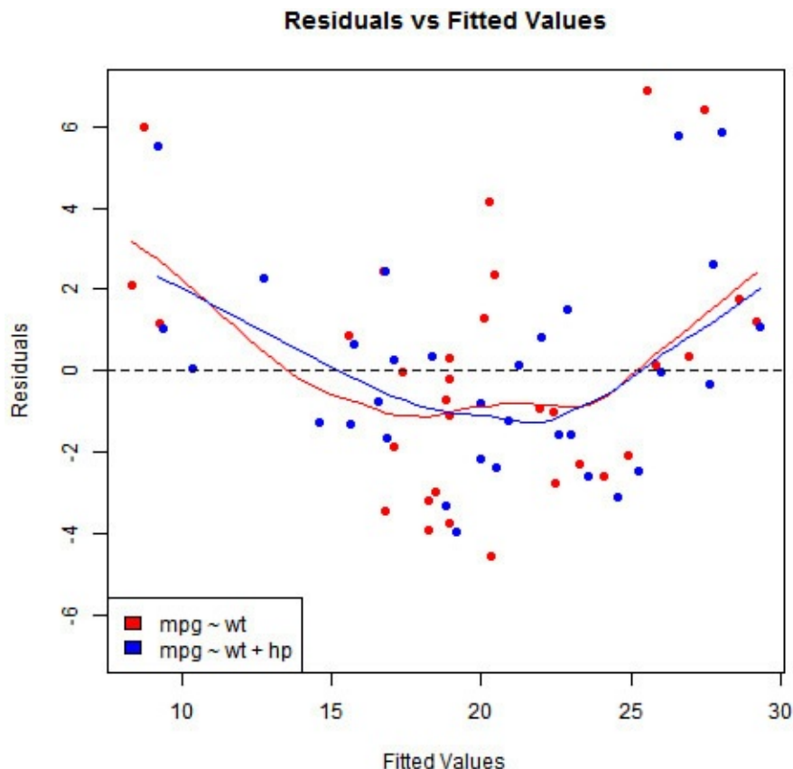
FIGURE 16.5 Scatter plot of residuals vs. fitted values for two linear models
