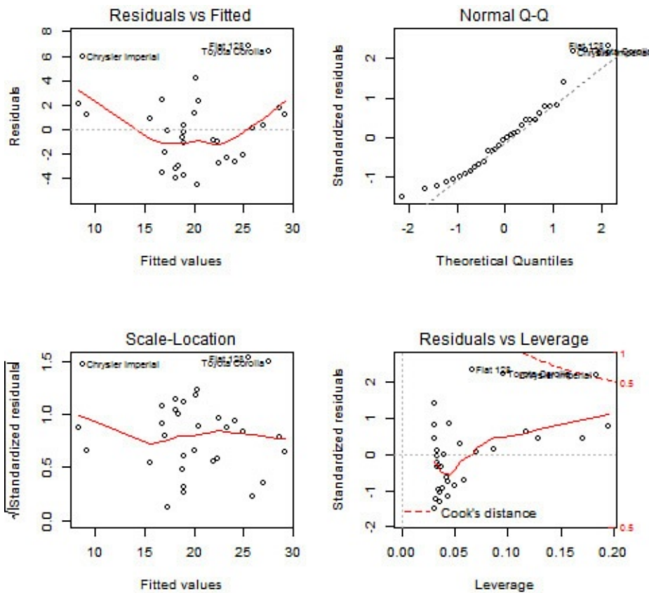
FIGURE 16.2 Diagnostic plots for linear regression
