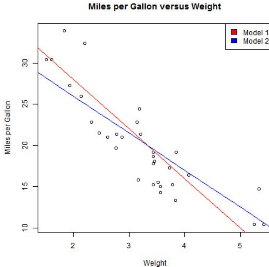
FIGURE 17.4 Plot of miles per gallon versus weight with two candidate models
