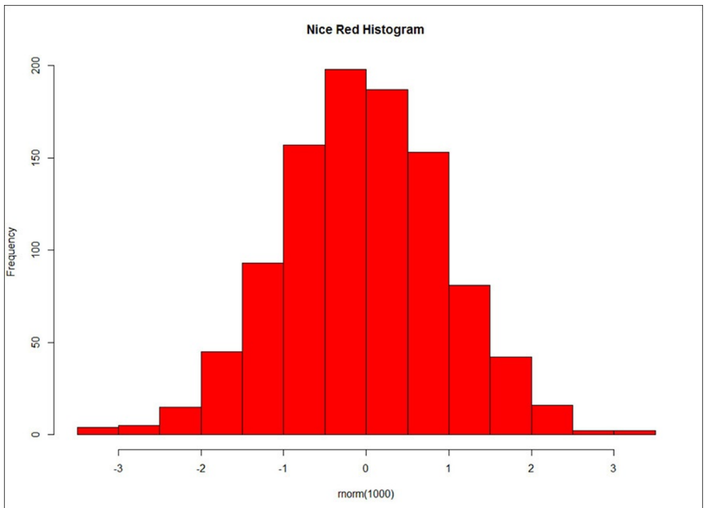
FIGURE 8.1 Histogram of samples from a normal distribution
