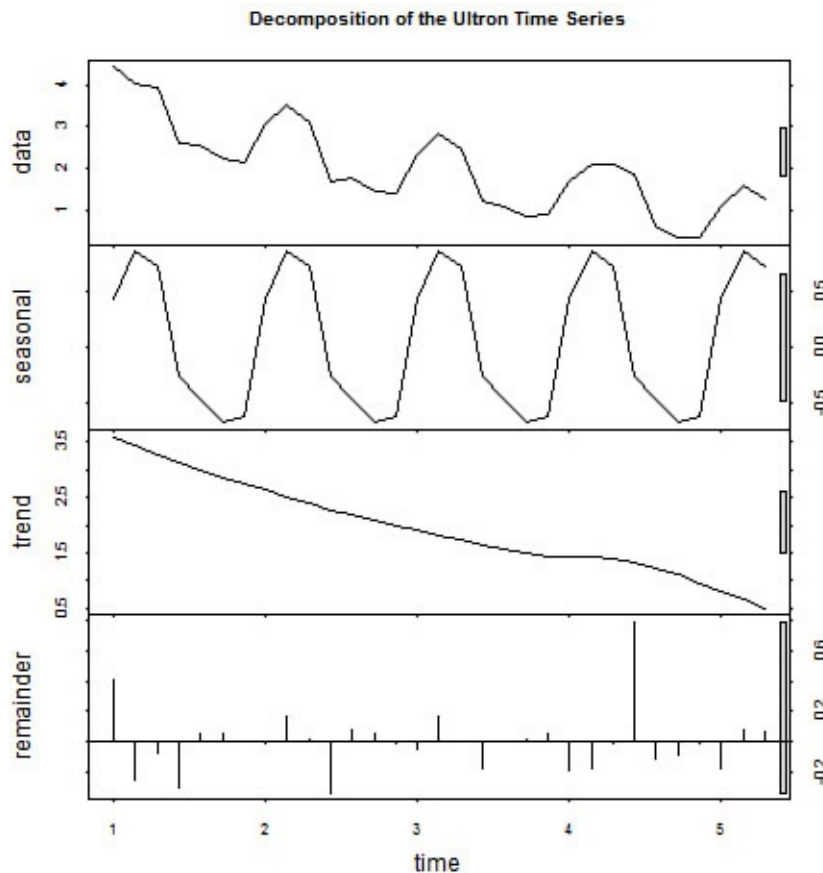
FIGURE 17.17 Decomposition of (logged) daily grossing of Avengers: Age of Ultron
