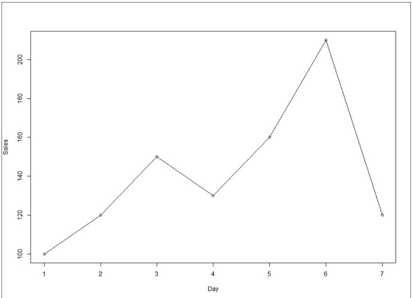
FIGURE 8.4 Simple line plot of Sales versus Day
