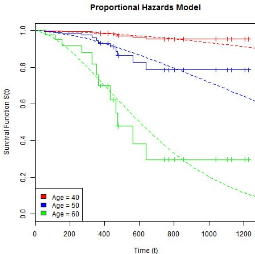
FIGURE 17.14 Estimated survival for different ages using Proportional Hazards model
