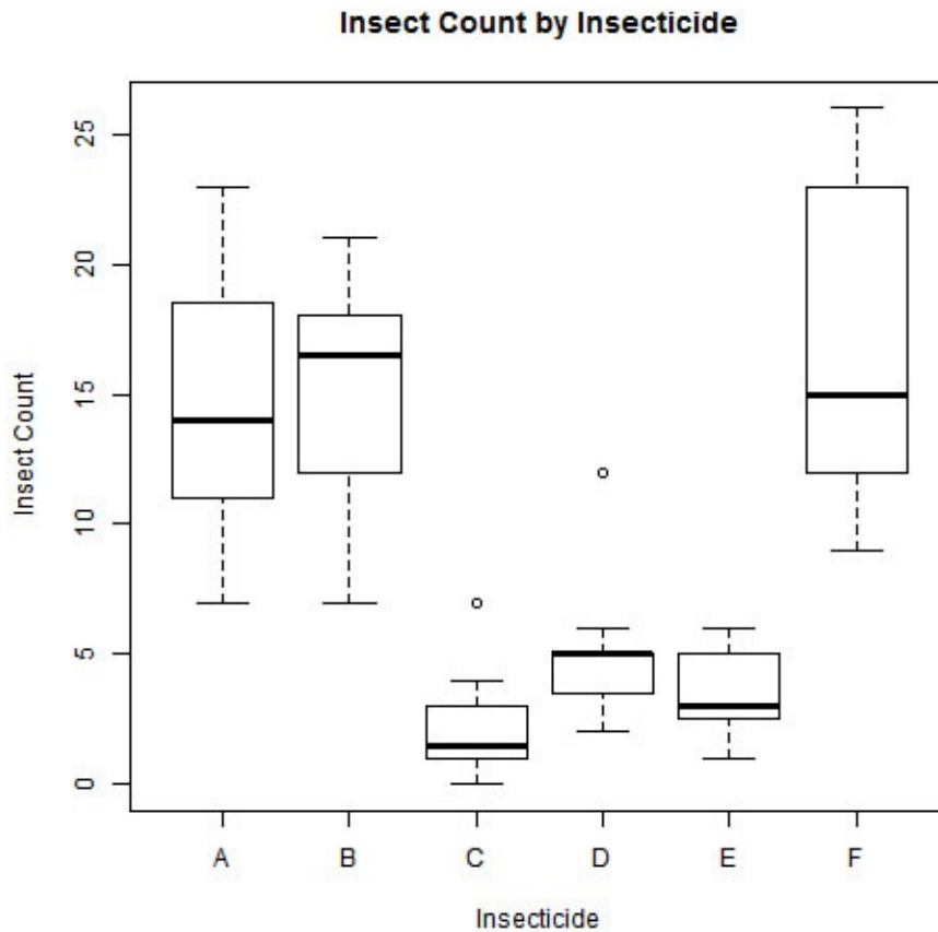
FIGURE 17.3 Plot of InsectSprays data
