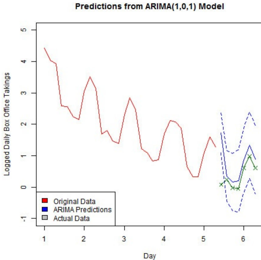
FIGURE 17.24 Time series predictions from ARIMA Model
