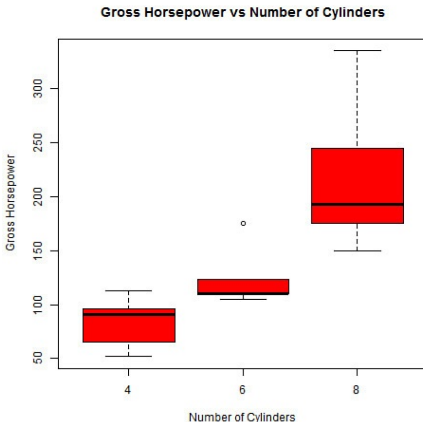
FIGURE 16.9 Gross horsepower vs. number of cylinders ( cyl versus hp )
