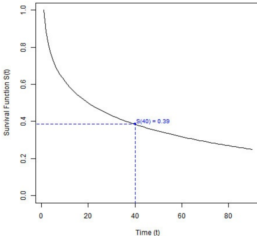
FIGURE 17.9 Example of a Survival Function
