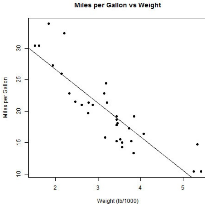
FIGURE 16.4 Scatter plot of mpg versus wt with overlaid regression line
