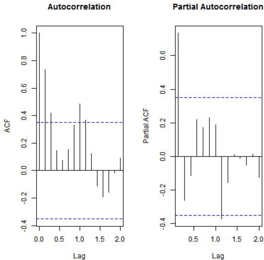
FIGURE 17.21 Correlograms of logged daily box office takings for Avengers: Age of Ultron
