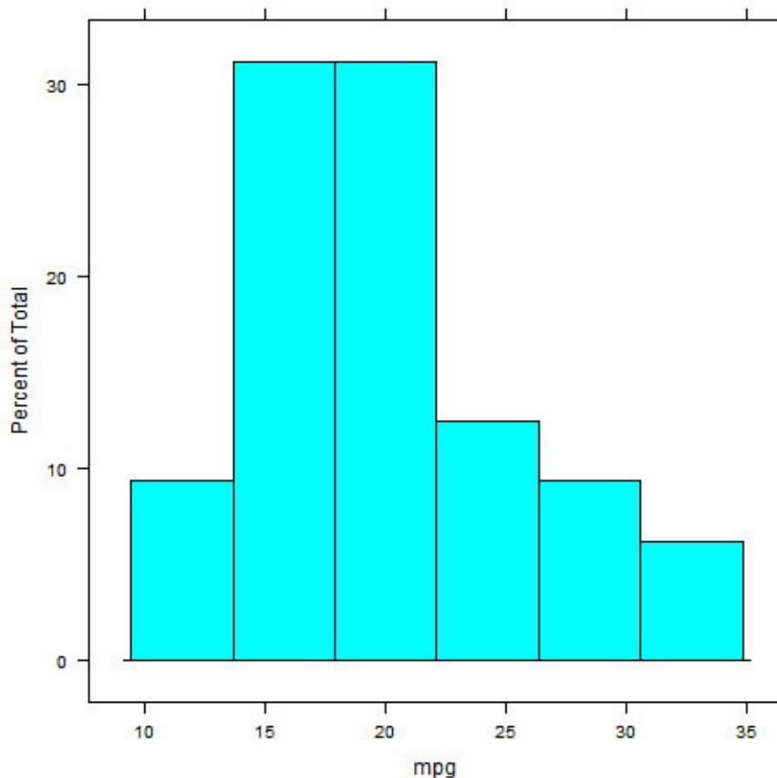
FIGURE 15.2 A histogram of mpg
