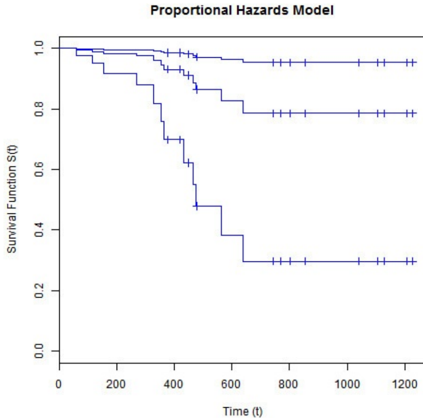
FIGURE 17.13 Estimated survival using Proportional Hazards model
