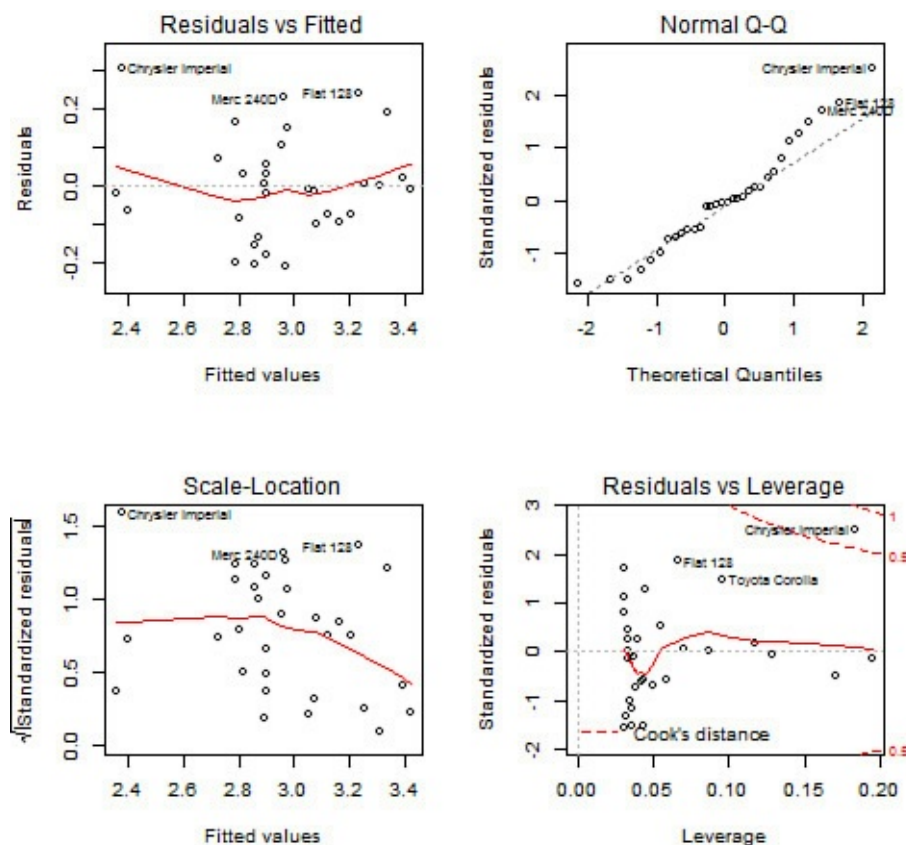
FIGURE 16.11 Diagnostic plots for log model fit
