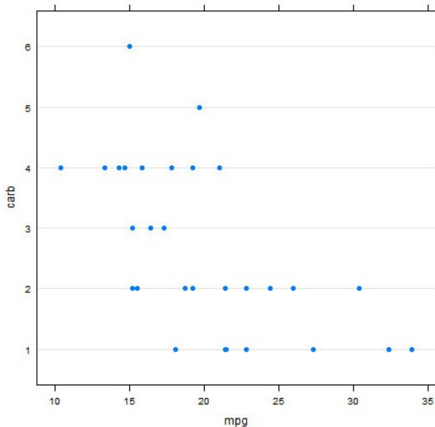
FIGURE 15.4 A dot plot of carb vs mpg
