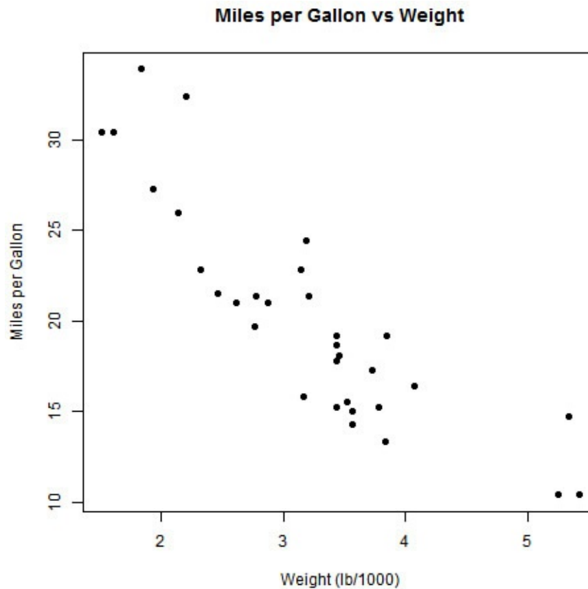
FIGURE 16.1 A scatter plot of mpg versus wt
