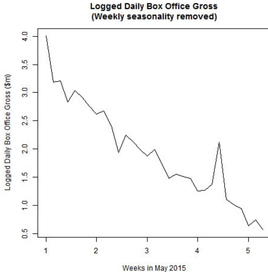
FIGURE 17.18 Logged daily grossing of Avengers: Age of Ultron with seasonality removed
