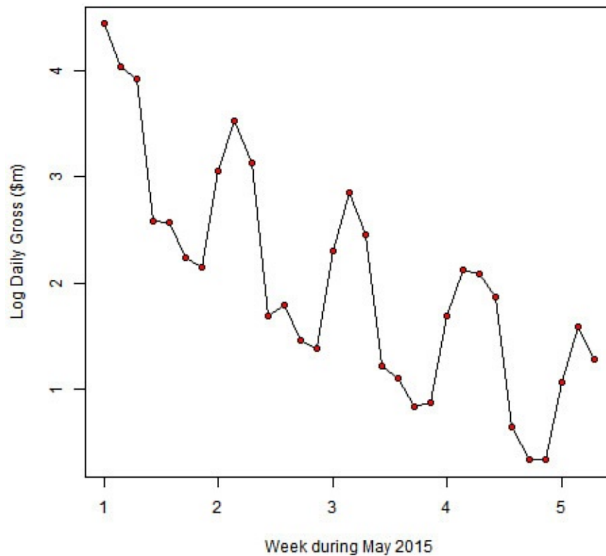
FIGURE 17.16 Time series plot of (logged) daily grossing of Avengers: Age of Ultron
