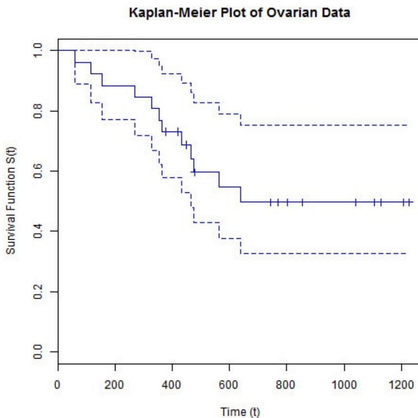
FIGURE 17.10 Kaplan-Meier plot of ovarian data
