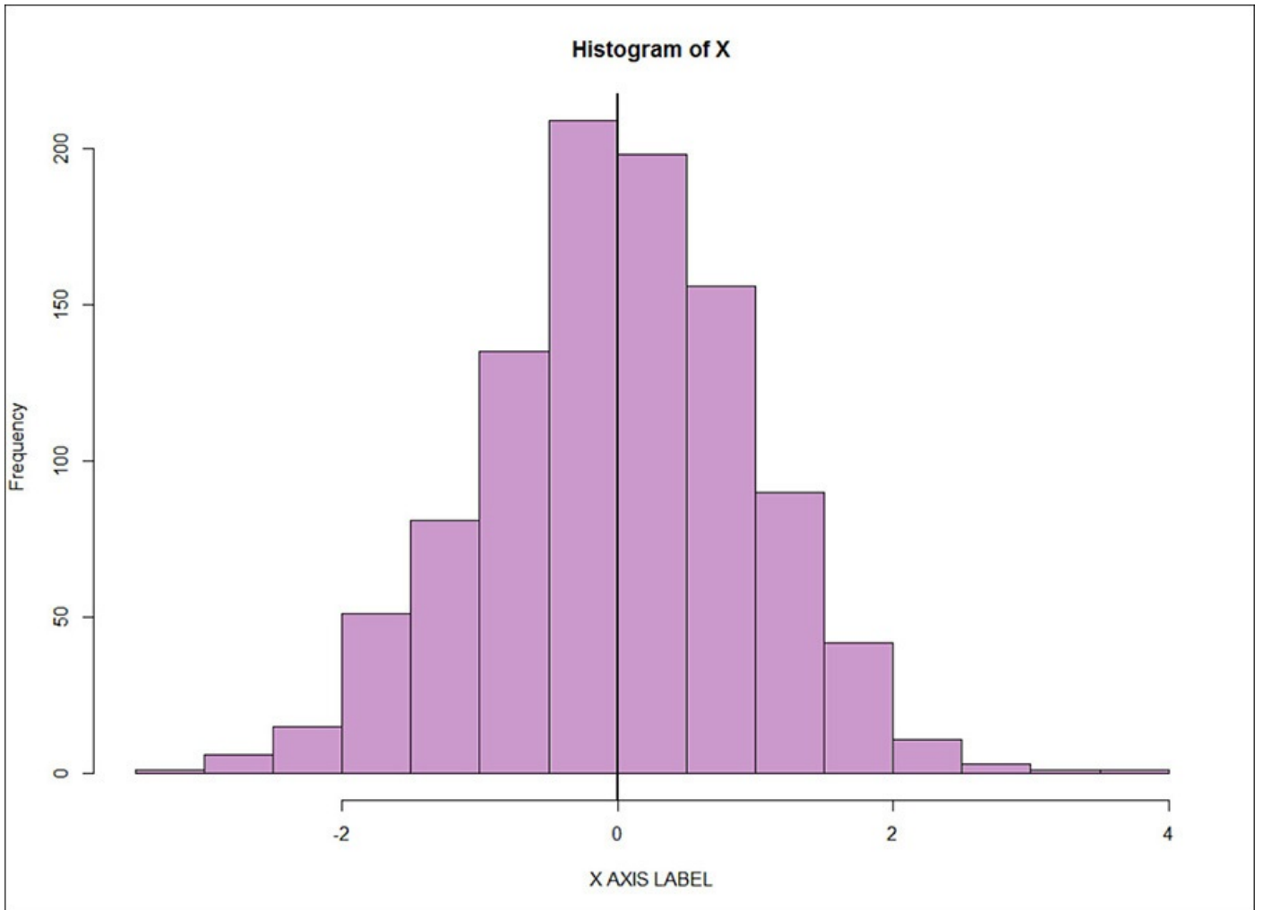
FIGURE 8.3 Plum-colored histogram created with histFun
