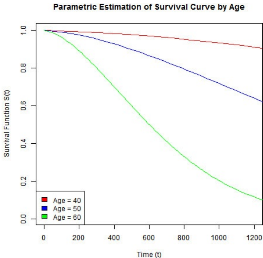
FIGURE 17.12 Estimated survival by age
