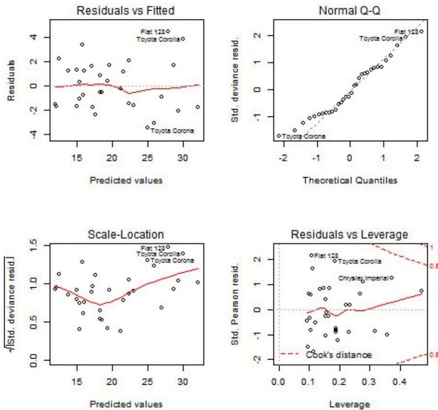
FIGURE 17.1 Diagnostic plots for GLM
