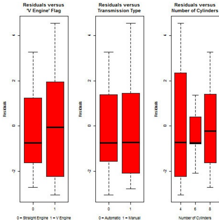
FIGURE 16.8 Model residuals versus vs, am, and cyl
