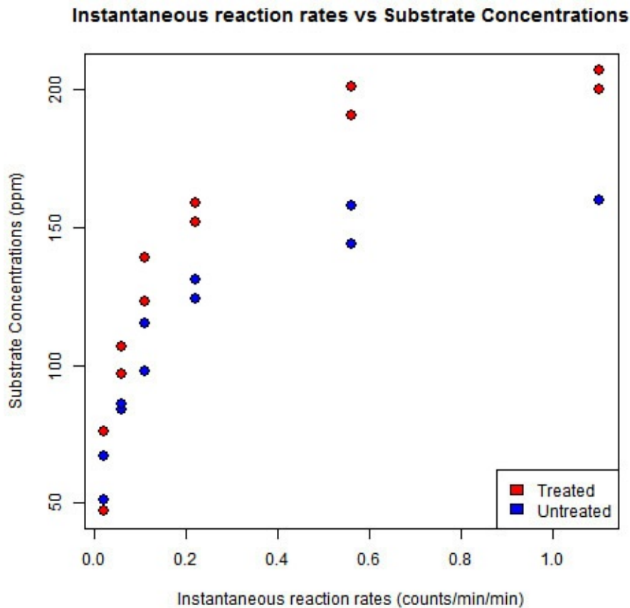
FIGURE 17.5 Plot of reaction rates versus concentration from the Puromycin data
