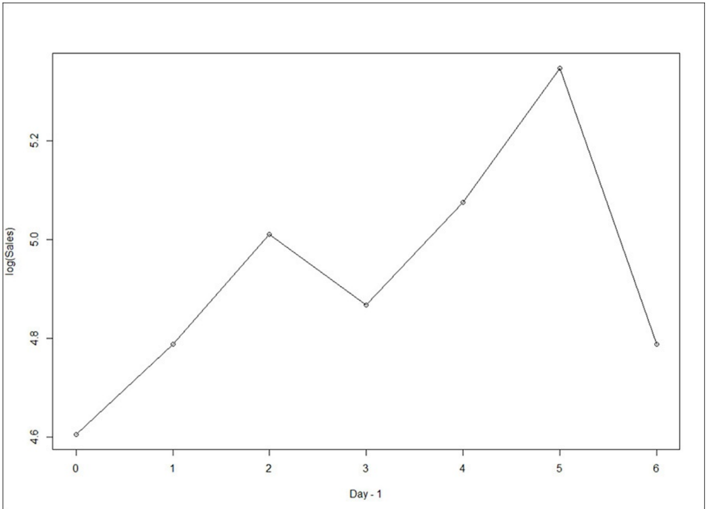
FIGURE 8.5 Simple line plot of \log(\text{Sales}) versus “Day – 1”
