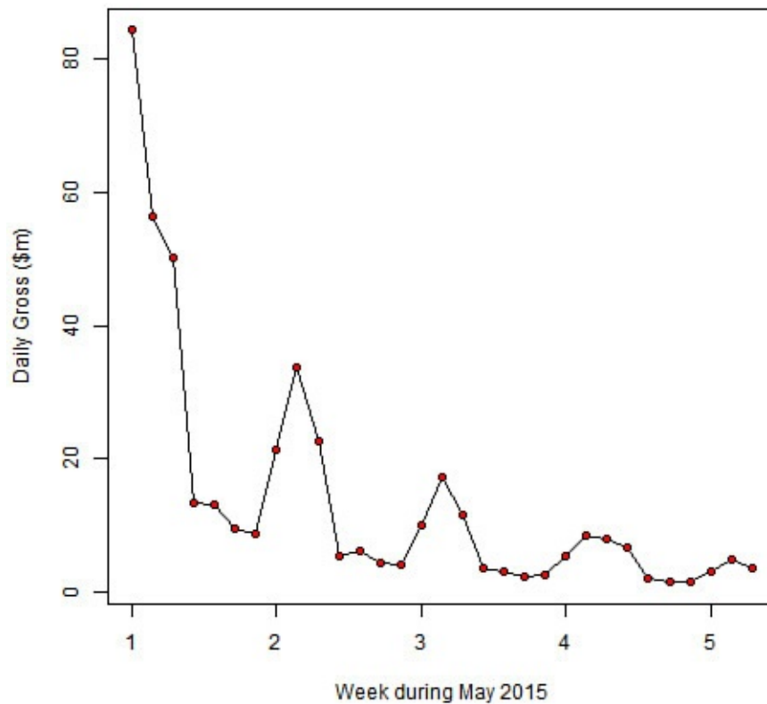
FIGURE 17.15 Time series plot of daily grossing of Avengers: Age of Ultron
