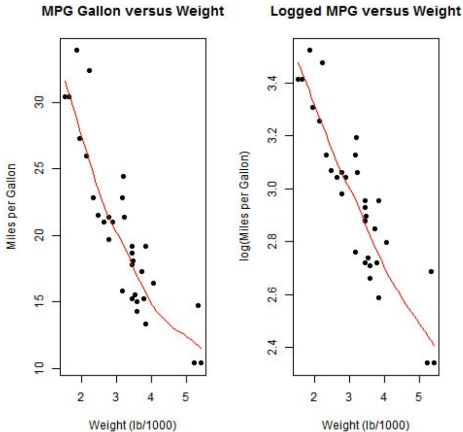
FIGURE 16.10 Scatter plots of miles per gallon and logged miles per gallon versus weight
