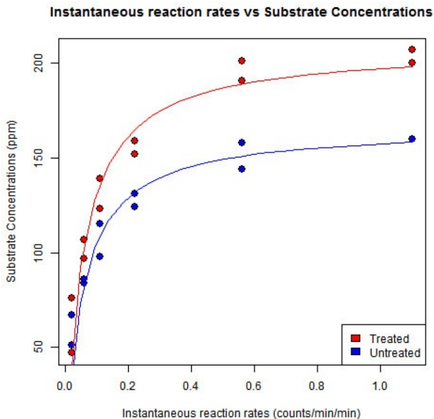
FIGURE 17.8 Plot of reaction rates versus concentration with Nonlinear model fit
