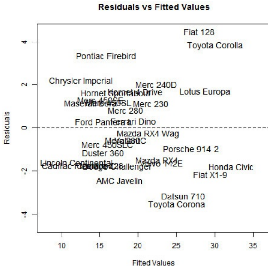
FIGURE 17.2 Plot of residuals versus fitted values for GLM
