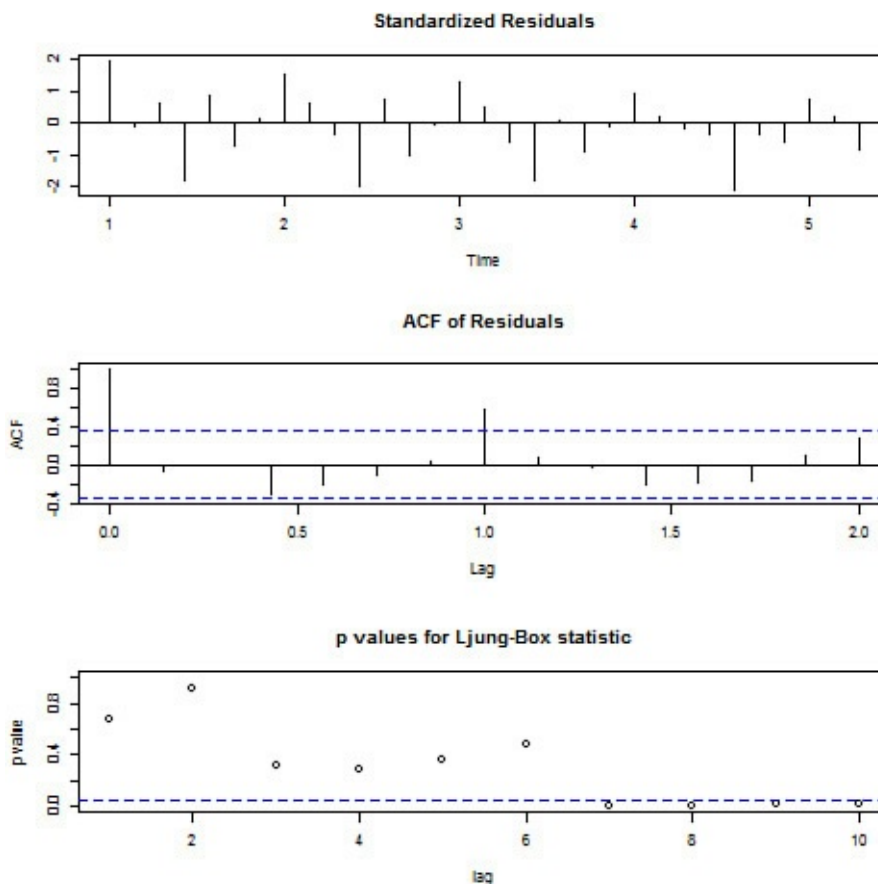
FIGURE 17.22 Diagnostic plots from ARIMA (1, 0, 1) fit
