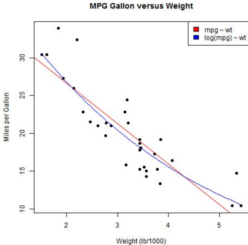
FIGURE 16.12 Scatter plot of miles per gallon versus weight, overlaid with two models
