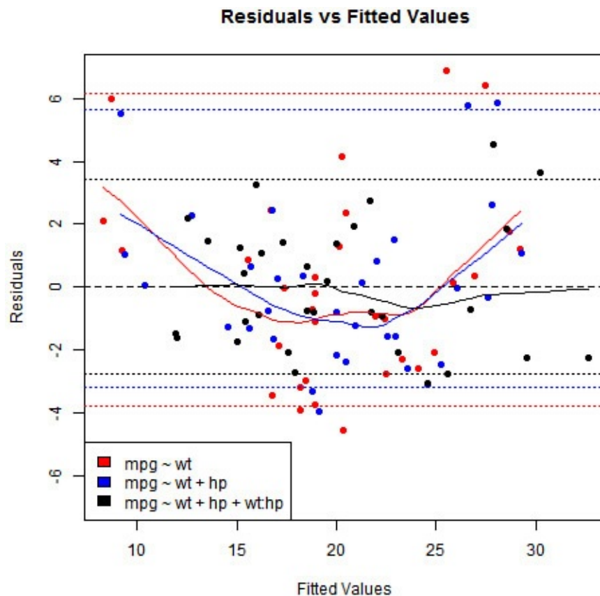
FIGURE 16.7 Scatter plot of residuals vs fitted values for three linear models
