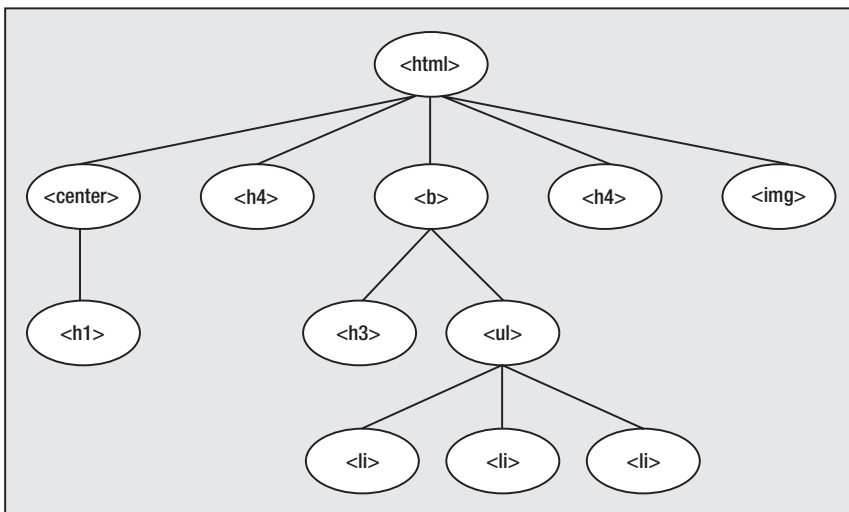
Figure 13-3. If a document is well-formed, the relationship between the elements is a hierarchical one, with each descendent contained between its parent's start and end tags.
