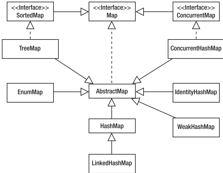
Figure 4-2. The Map interface and its associated classes aren't part of the same hierarchy as the other components you've seen.
