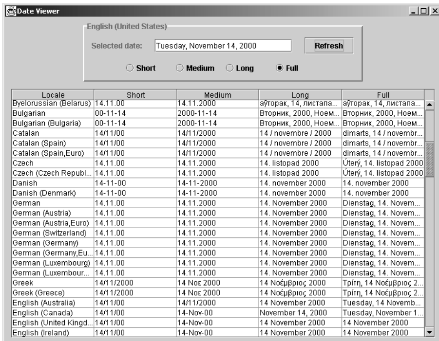
Figure 12-3. Some of the many different date formats associated with various locales
