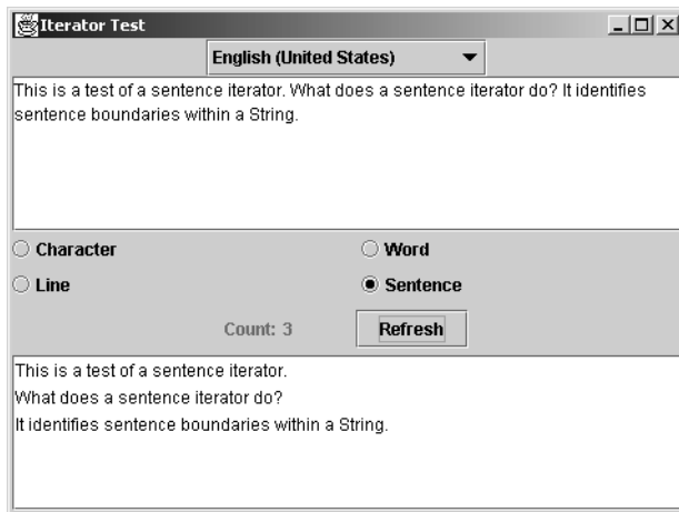
Figure 12-6. BreakIterator contains sophisticated logic for identifying sentence breaks.
