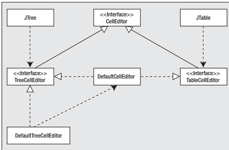
Figure 7-18. The relationships between the classes and interfaces involved in editing tree and table cells
