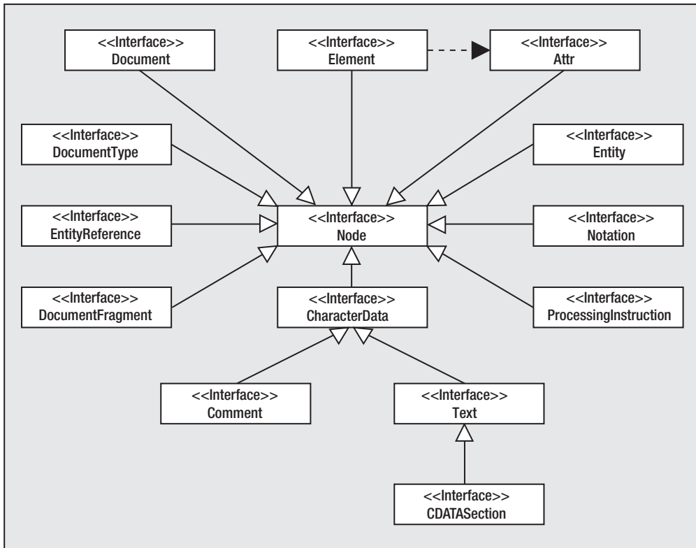
Figure 13-5. A class diagram that illustrates the relationships between the classes and interfaces used by the DOM parser in JAXP
