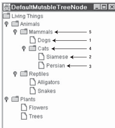
Figure 7-10. A more complex example of how depth-first enumeration works
