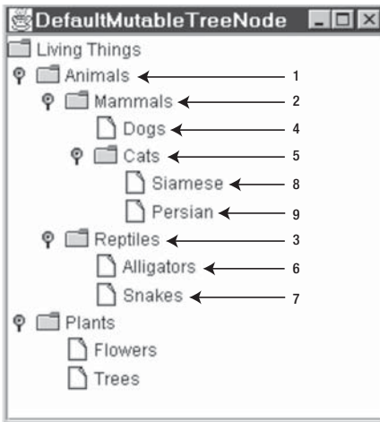
Figure 7-11. Breadth-first enumeration traverses a set of nodes based on their level.
