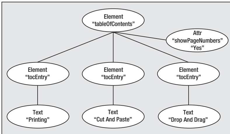
Figure 13-6. An example of the hierarchical nature of the elements with a DOM tree
