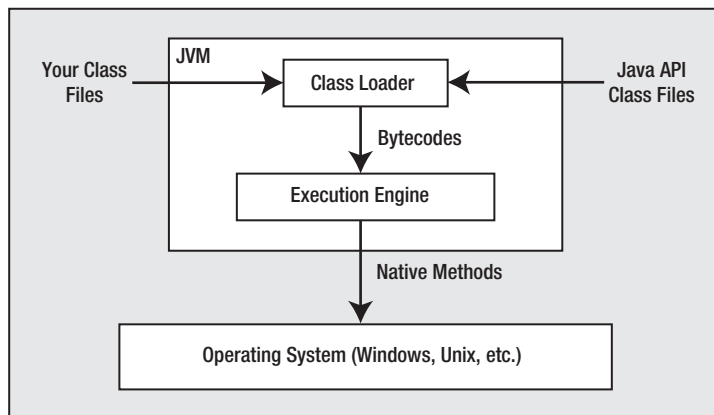
Figure 1-2. Role of the JVM
