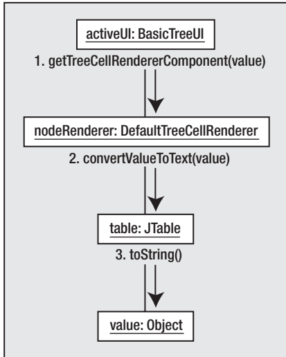
Figure 7-15. The classes and methods used by default to render the nodes in a tree
