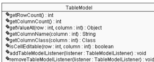
Figure 6-2. A simple class diagram showing the methods defined in TableModel
