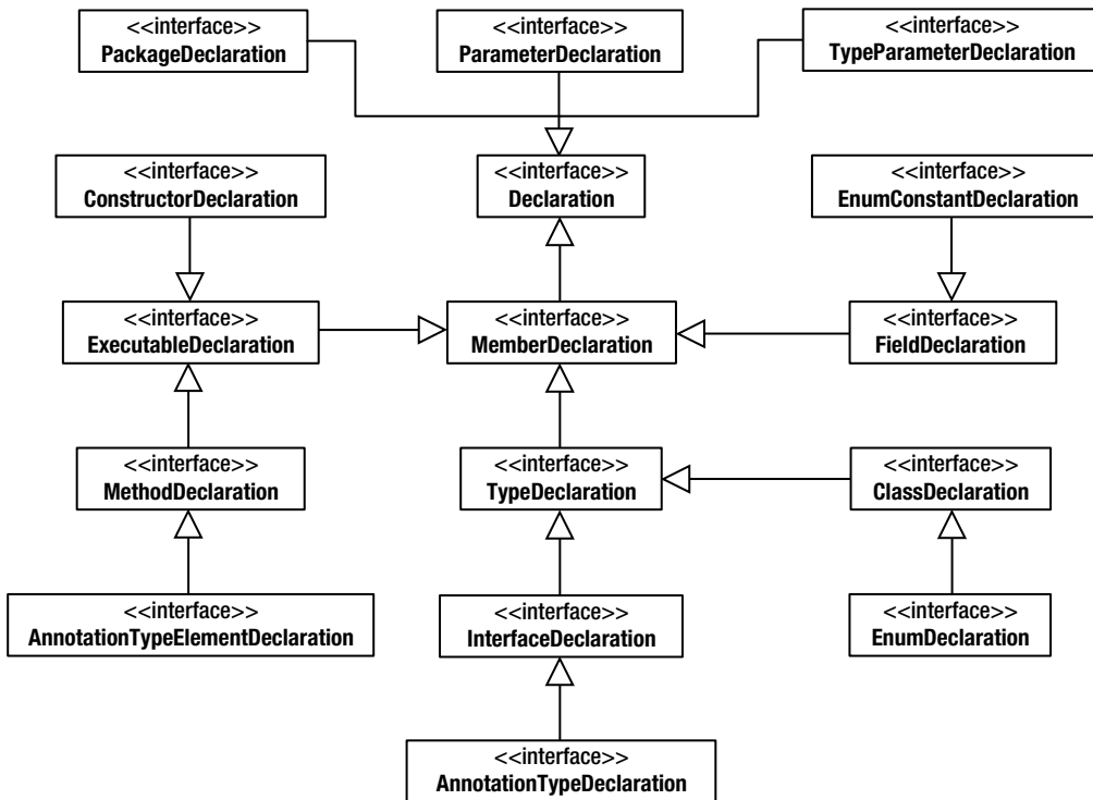
Figure 14-3. The com.sun.mirror.declaration package contains a variety of interfaces used to represent the various source code elements.
