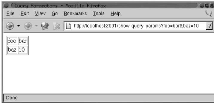
Figure 26-4. http://localhost:2001/show-query-params?foo=bar&baz=10
