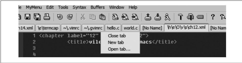
Figure 11-4. Example of gvim tabs and tabbed editing
