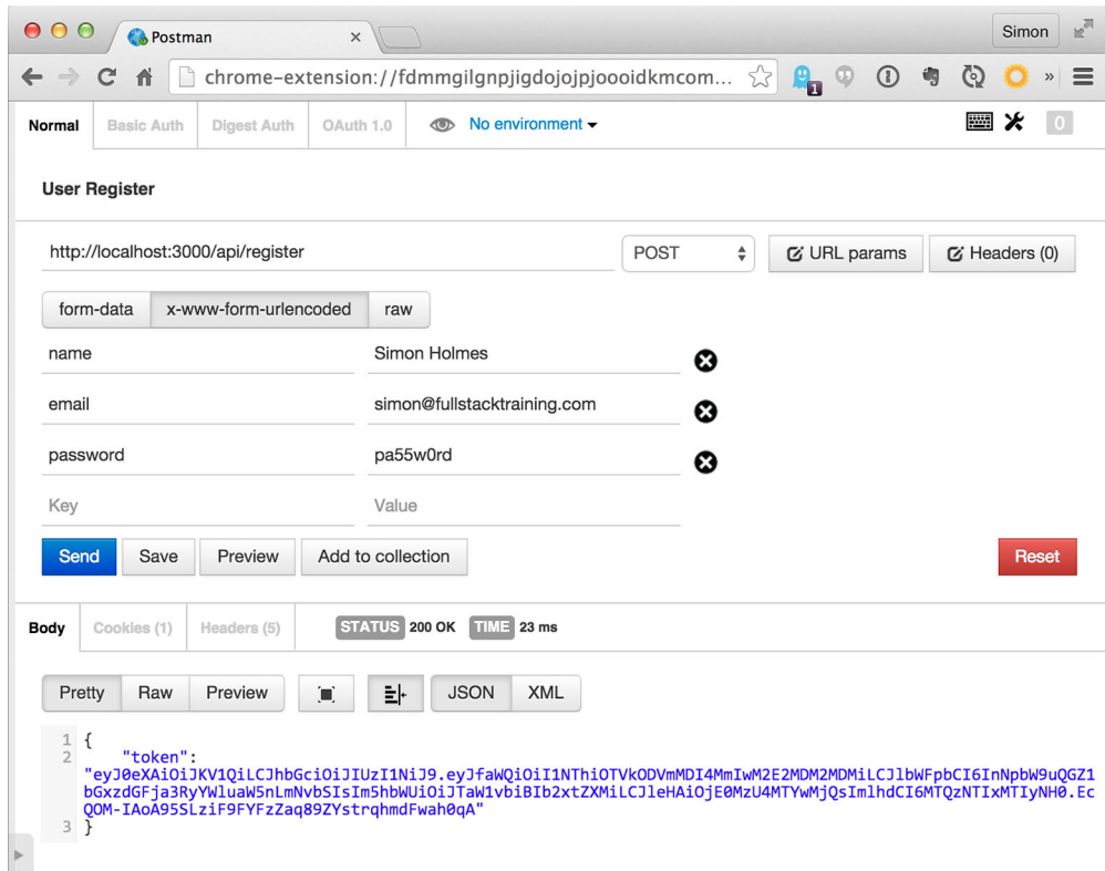
Figure 11.9 Trying out the /api/register endpoint in Postman, returning a JWT when successful
