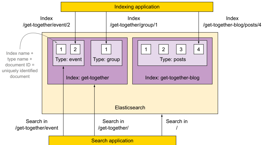
Figure 2.2 Logical layout of data in Elasticsearch: how an application sees data
