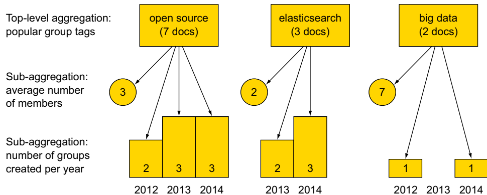
Figure 7.2 The terms bucket aggregation allows you to nest other aggregations within it.
