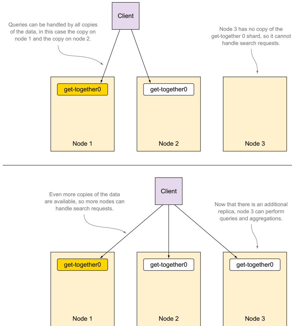
Figure 9.9 Additional replicas handling search and aggregations
