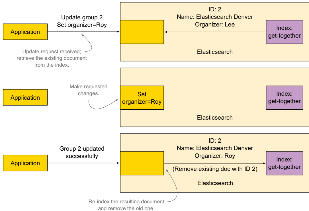
Figure 3.3 Updating a document involves retrieving it, processing it, and re-indexing it while overwriting the previous document.
