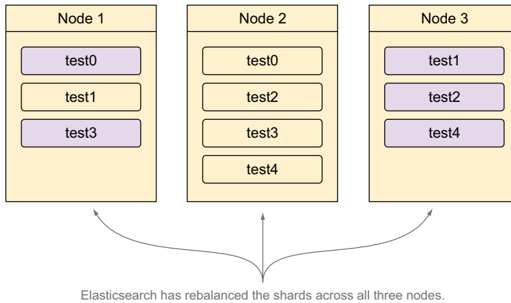
Figure 9.2 Shard allocation for the test index with three Elasticsearch nodes
