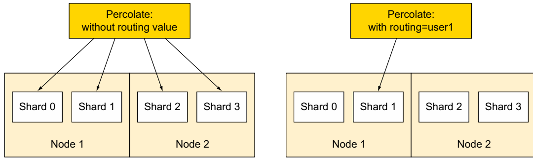
Figure E.4 A percolate request with routing reduces the number of queries and also hits fewer shards.
