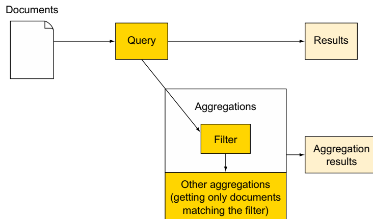
Figure 7.13 The filter aggregation restricts query results for aggregations nested under it.
