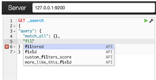
Figure D.8 Autocompletion of REST calls
