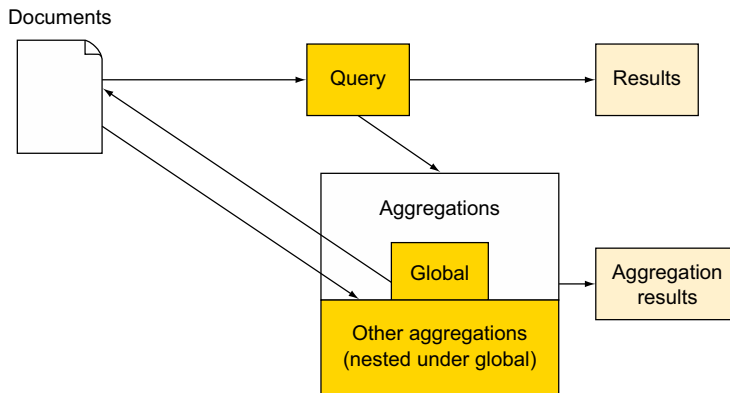
Figure 7.12 Nesting aggregations under the global aggregation makes them run on all documents.
