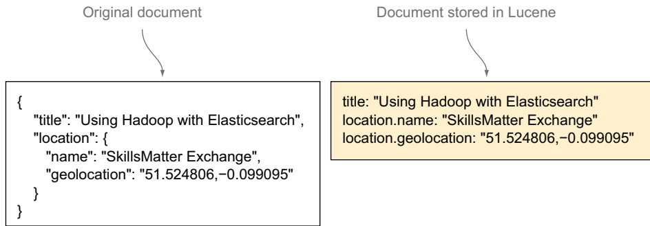
Figure 8.6 JSON hierarchical structure stored as a flat structure in Lucene
