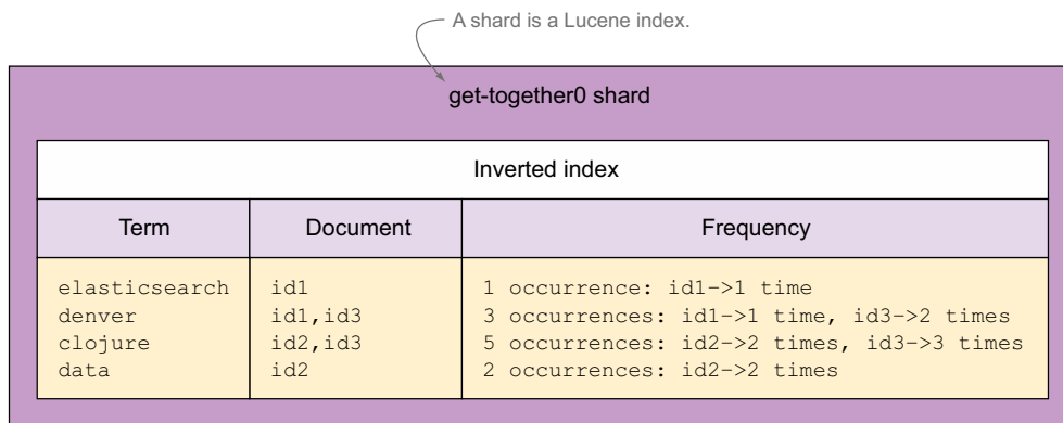
Figure 2.5 Term dictionary and frequencies in a Lucene index
