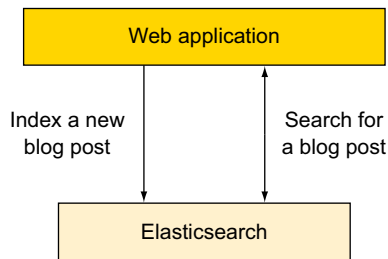
Figure 1.2 Elasticsearch as the only back end storing and indexing all your data
