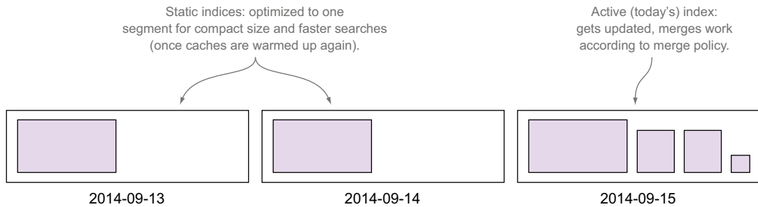
Figure 10.5 Optimizing makes sense for indices that don't get updates.
