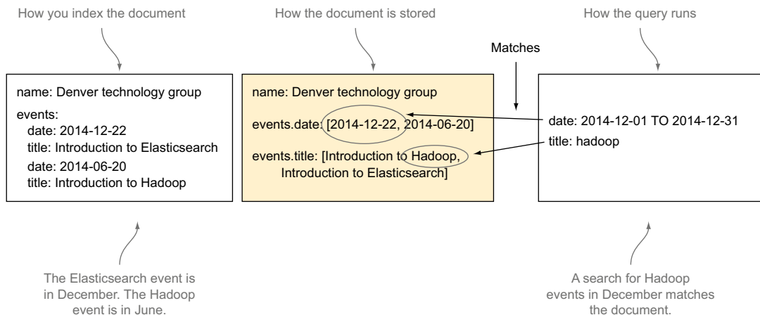
Figure 8.1 Inner object boundaries aren't accounted for when storing, leading to unexpected results.
