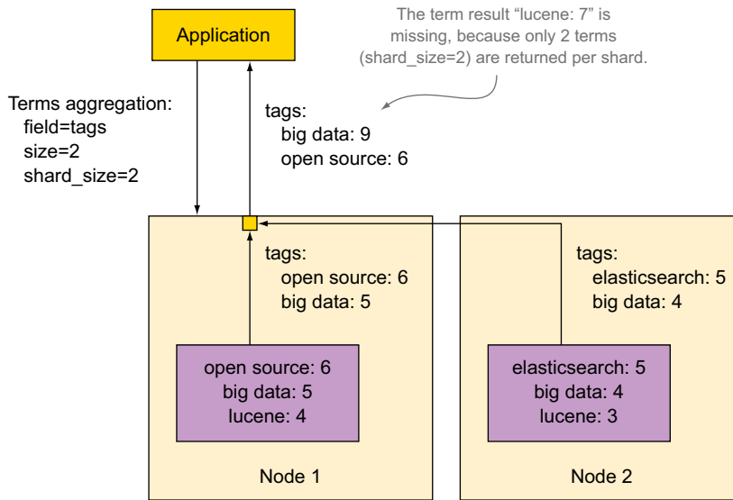
Figure 7.7 Sometimes the overall top X is inaccurate, because only the top X terms are returned per shard.
