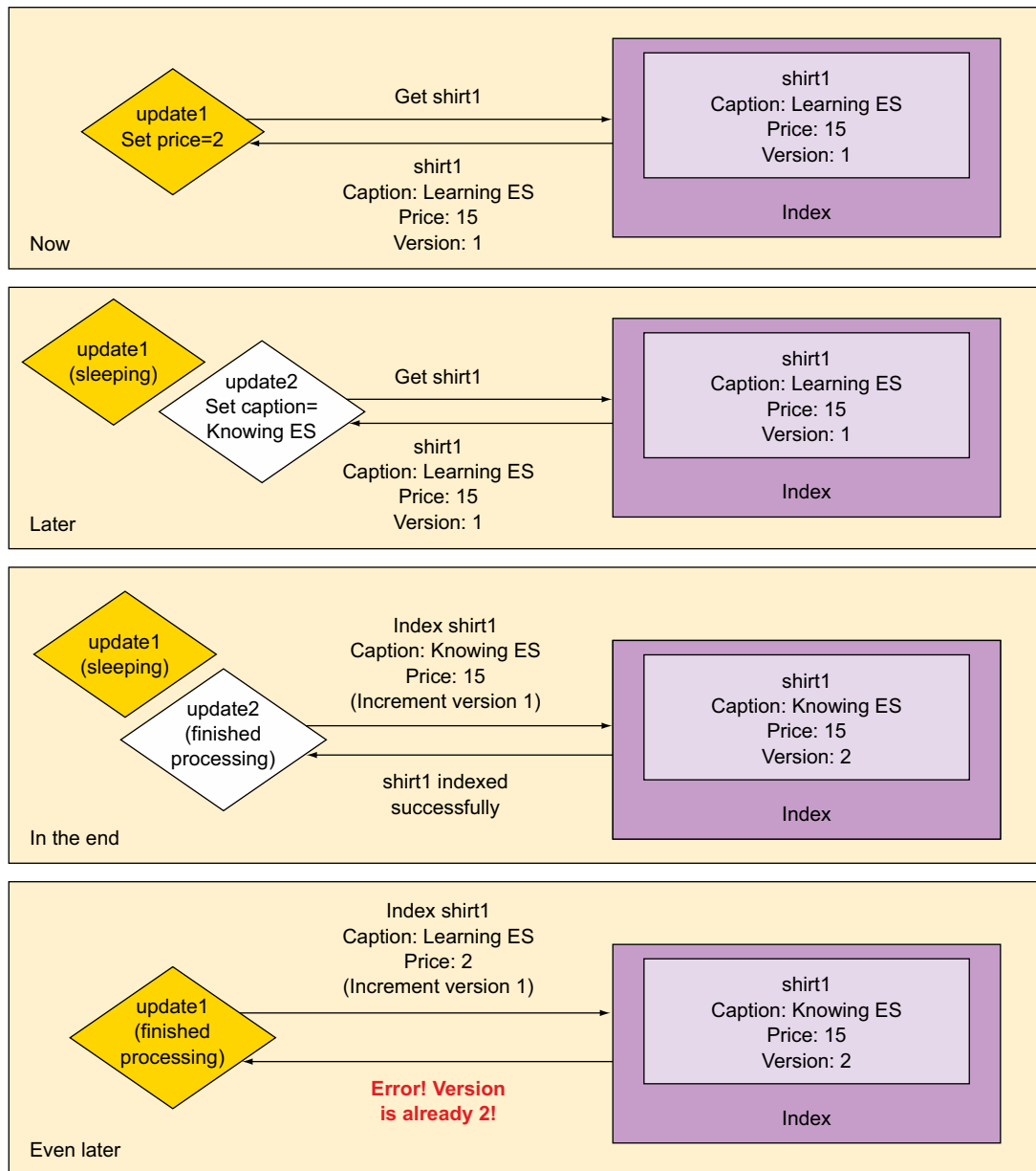
Figure 3.5 Concurrency control through versioning prevents one update from overriding another.
