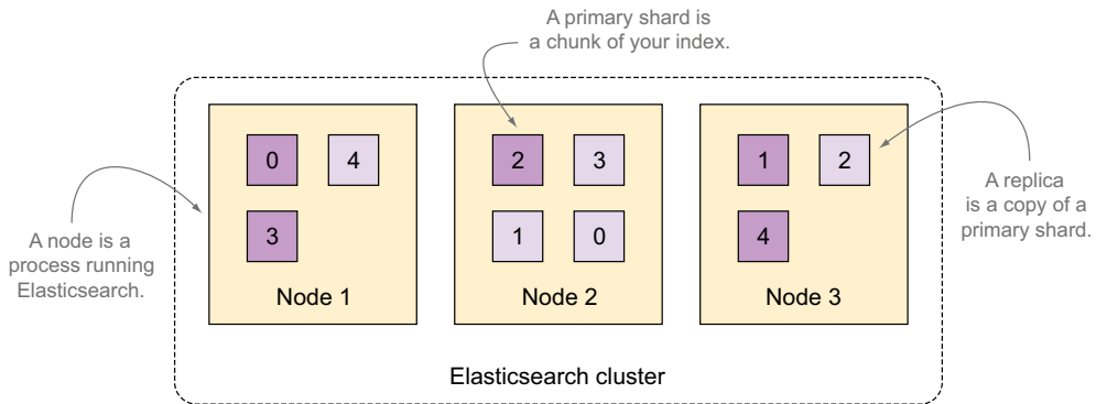
Figure 2.3 A three-node cluster with an index divided into five shards with one replica per shard
