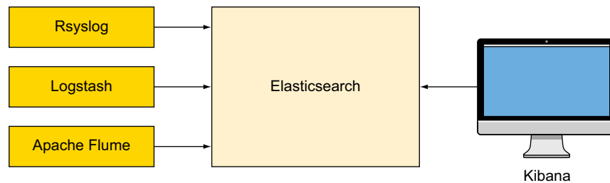
Figure 1.4 Elasticsearch in a system of logging tools that support Elasticsearch out of the box
