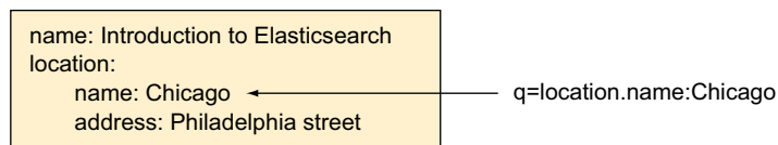
Figure 8.7 You can search in an object's field by specifying that field's full path.
