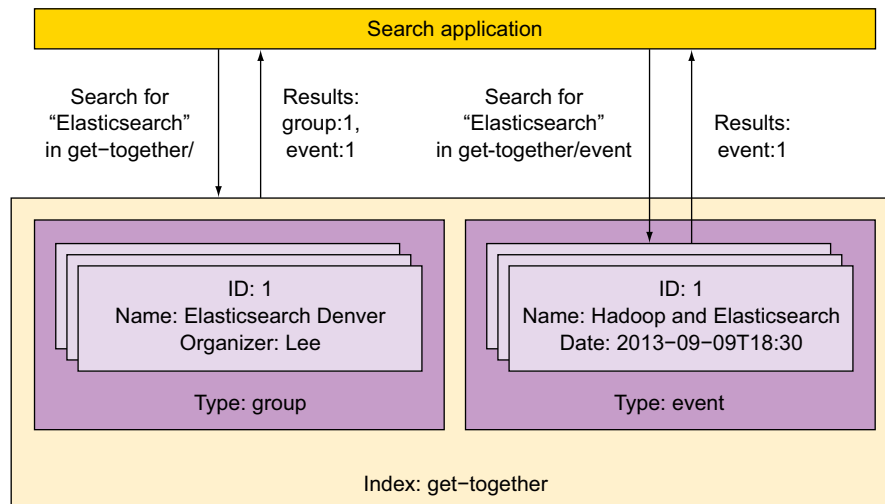
Figure 3.1 Using types to divide data in the same index; searches can run in one, multiple, or all types.
