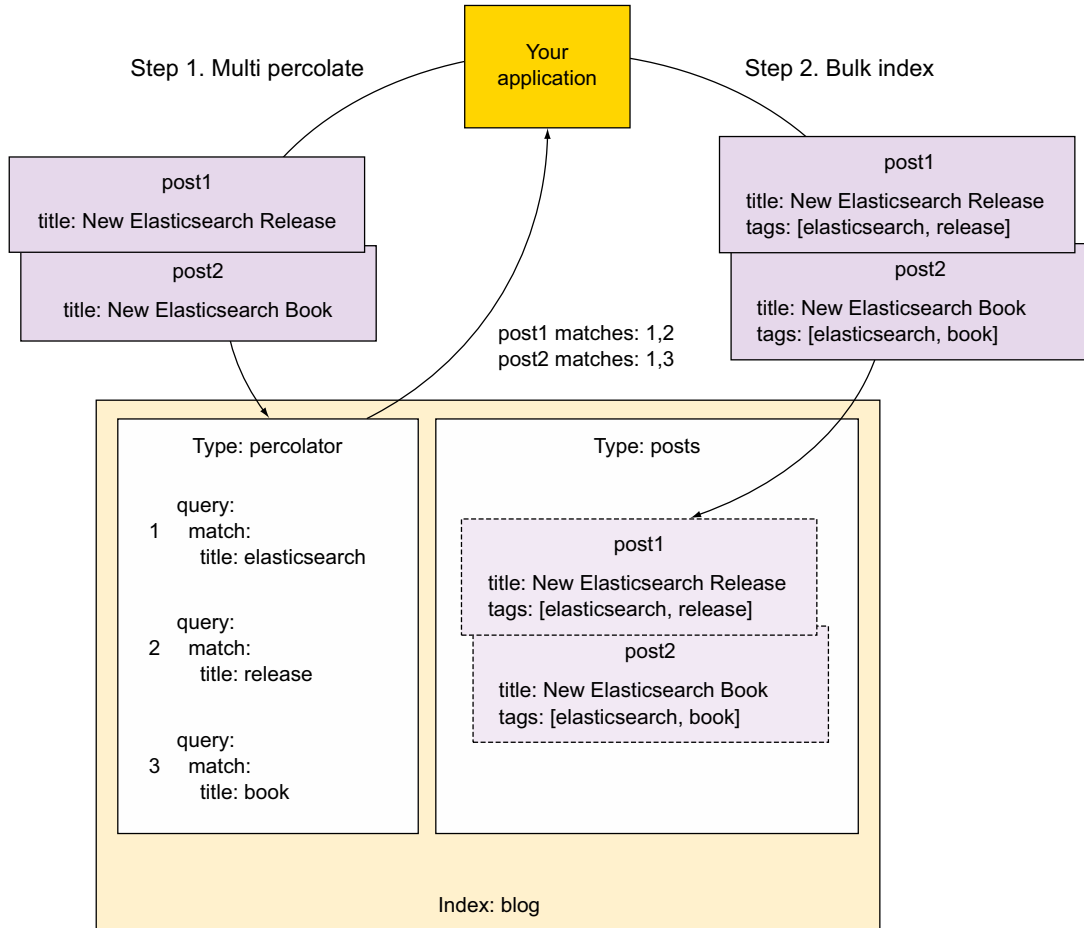
Figure E.3 Percolator for automated tagging. The multi percolate and bulk APIs reduce the number of requests. Before step 1, the percolation queries have been indexed. In step 1 you use the multi percolate API to find matching percolation queries. The application maps the IDs to the tags and adds them to the documents to index. In step 2 you use the bulk index API to index the documents.
