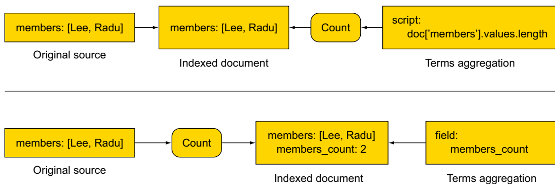
Figure 10.13 Counting members in a script or while indexing
