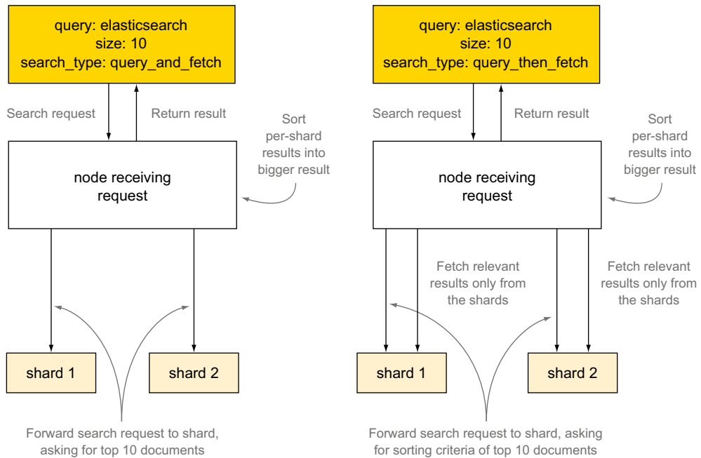
Figure 10.14 Comparison between query_and_fetch and query_then_fetch
