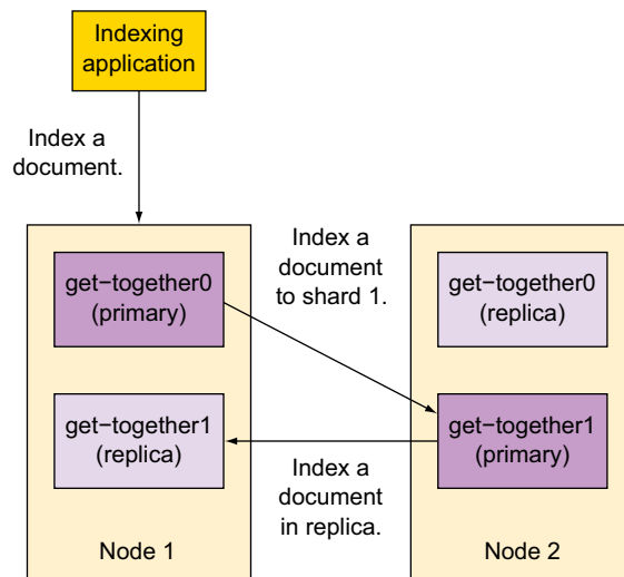
Figure 2.8 Indexing operation is forwarded to the responsible shard and then to its replicas.
