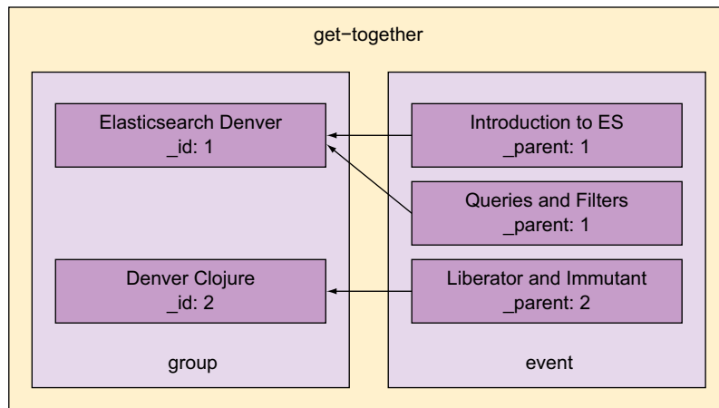
Figure 8.13 The _parent field of each child document is pointing to the _id field of its parent.
