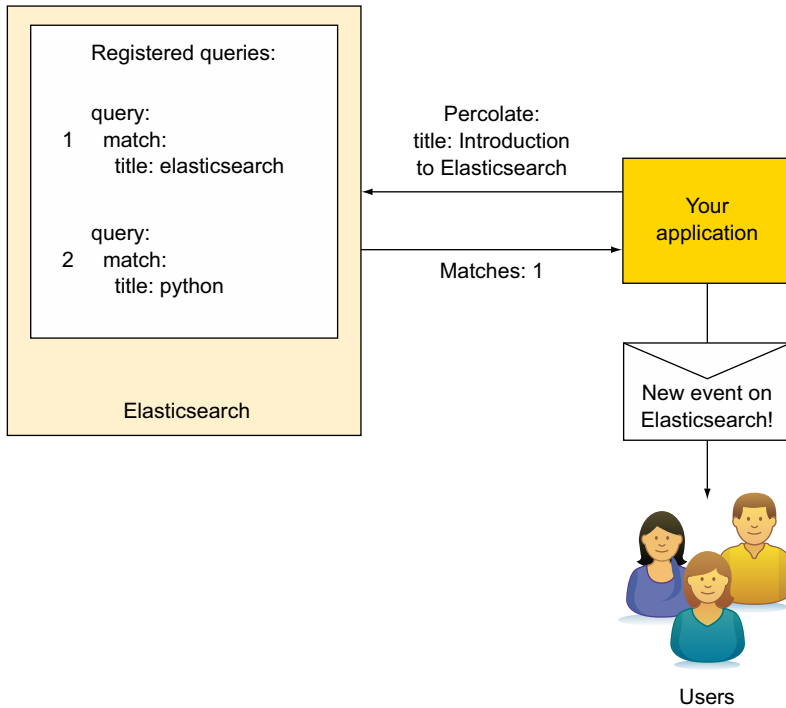
Figure E.1 Typical use case: percolating a document enables the application to send alerts to users if their stored queries match the document.
