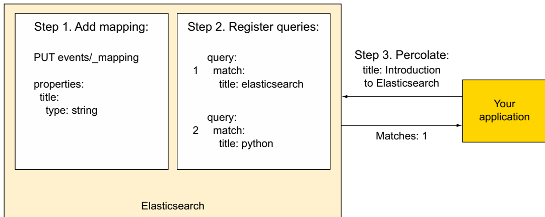
Figure E.2 You need a mapping and some registered queries in order to percolate documents.
