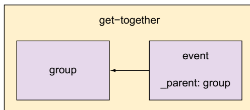
Figure 8.12 The relationship between events and groups as it's defined in the mapping
