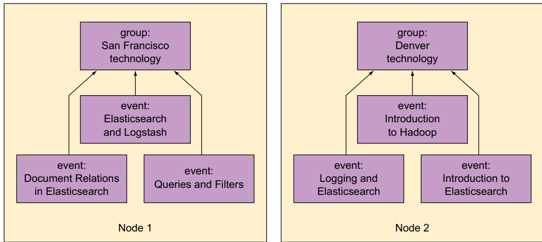
Figure 8.18 Nested/parent-child relations make sure all joins are local.
