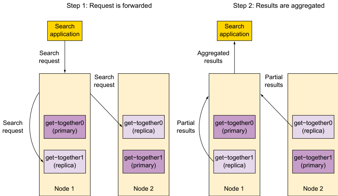
Figure 2.9 Search request is forwarded to primary/replica shards containing a complete set of data. Then results are aggregated and sent back to the client.
