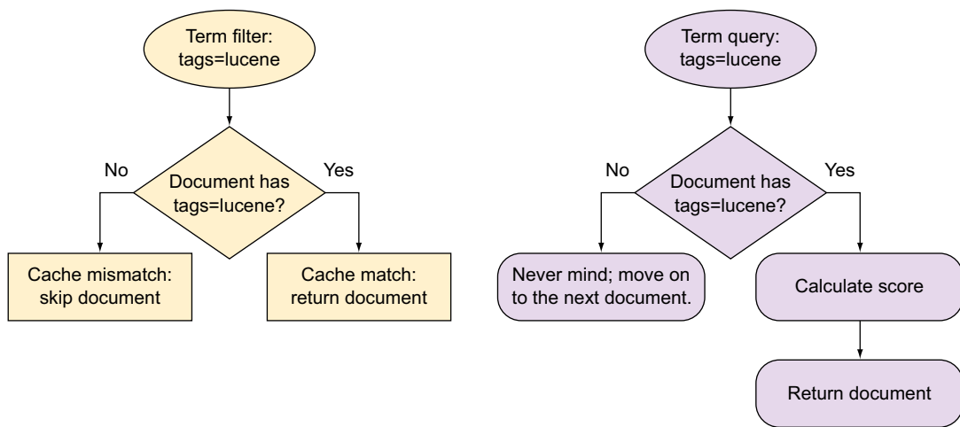
Figure 4.2 Filters require less processing and are cacheable because they don’t calculate the score.
