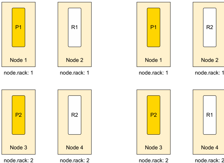
Figure 11.1 Cluster with default allocation settings
