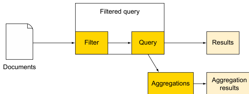
Figure 7.3 A filter wrapped in a filtered query runs first and restricts both results and aggregations.
