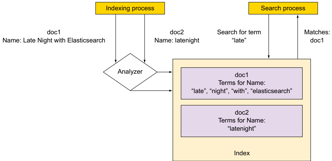
Figure 3.2 After the default analyzer breaks strings into terms, subsequent searches match those terms.
