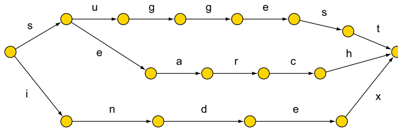
Figure F.6 In-memory FSTs help you get fast suggestions based on a prefix.
