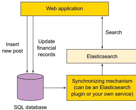
Figure 1.3 Elasticsearch in the same system with another data store
