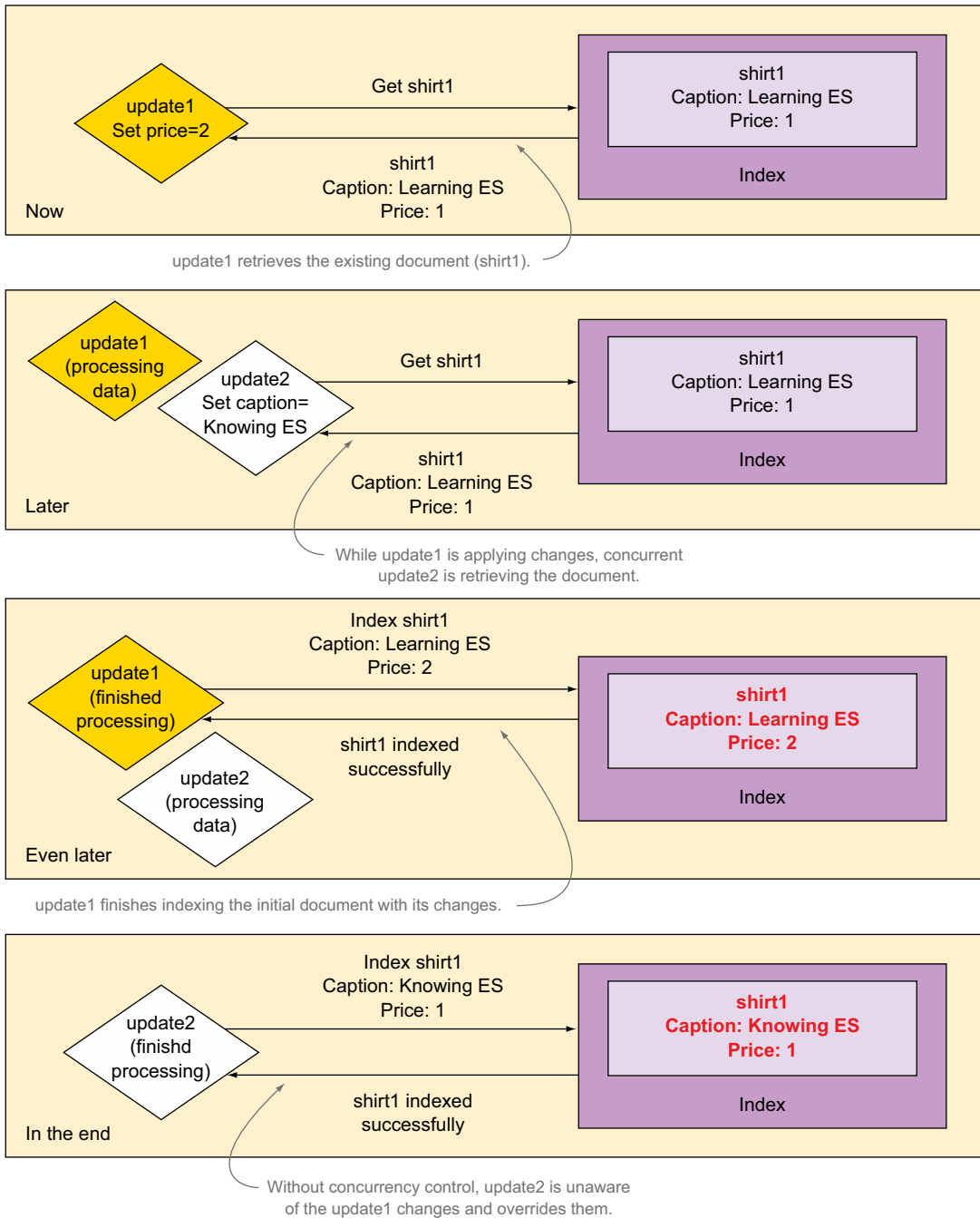
Figure 3.4 Without concurrency control, changes can get lost.
