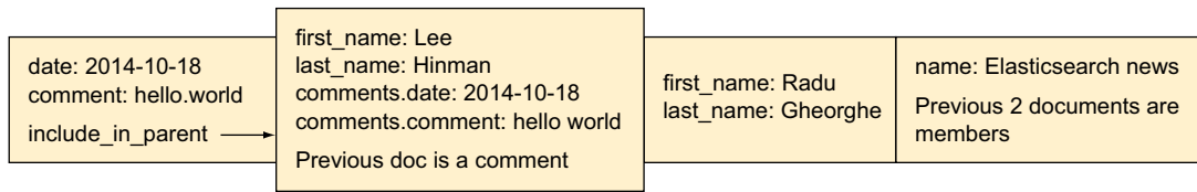
Figure 8.10 include_in_parent indexes a nested document's field into the immediate parent, too.
