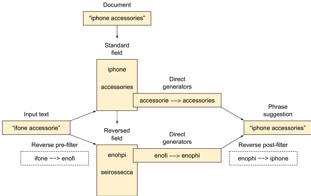
Figure F.4 Using filters and two direct generators to correct both prefix and suffix typos
