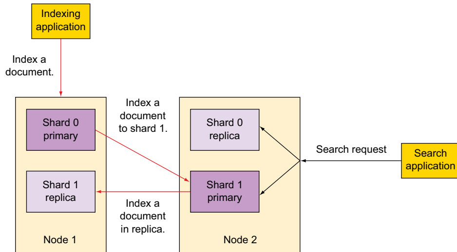
Figure 2.4 Documents are indexed to random primary shards and their replicas. Searches run on complete sets of shards, regardless of their status as primaries or replicas.
