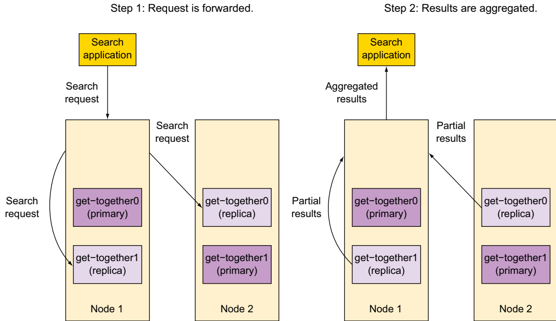
Figure 4.1 How a search request is routed; the index consists of two shards and one replica per shard. After locating and scoring the documents, only the top 10 documents are fetched.
