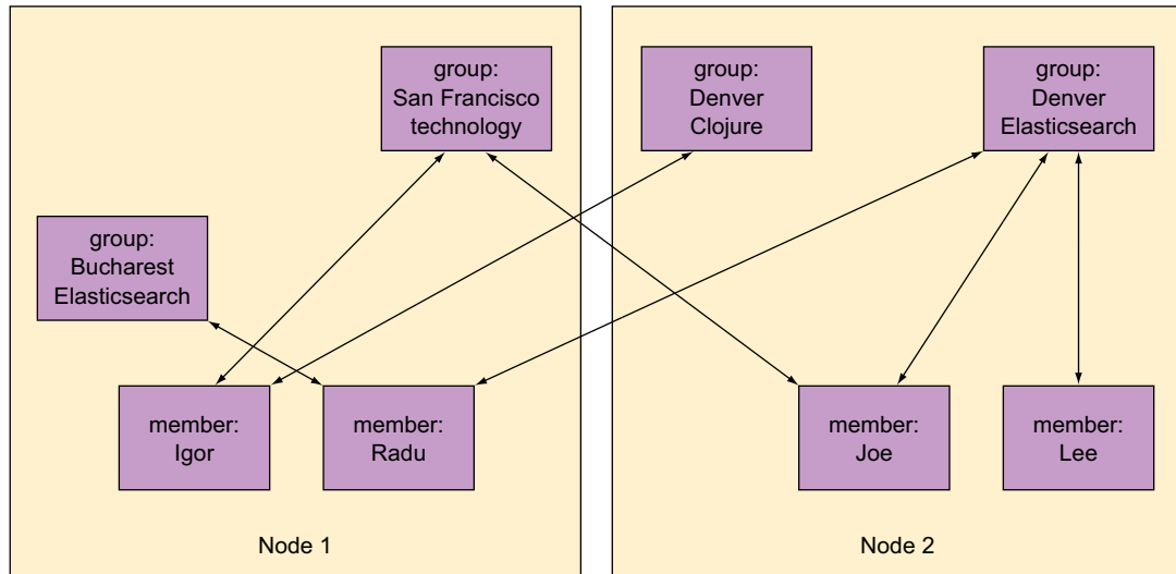
Figure 8.19 Many-to-many relationships can contain a huge amount of data, making local joins impossible.
