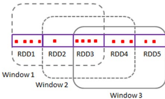
Figure 6-5. DStream windows
