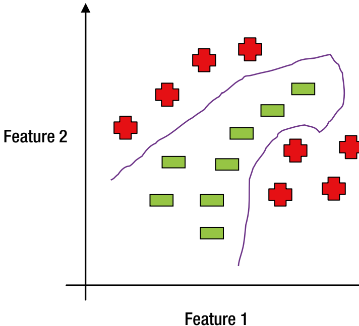
Figure 8-8. Non-linear Classifier
