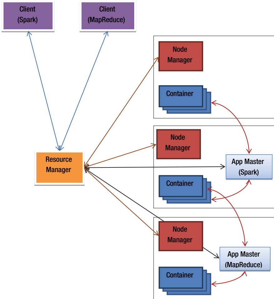
Figure 10-3. YARN architecture
