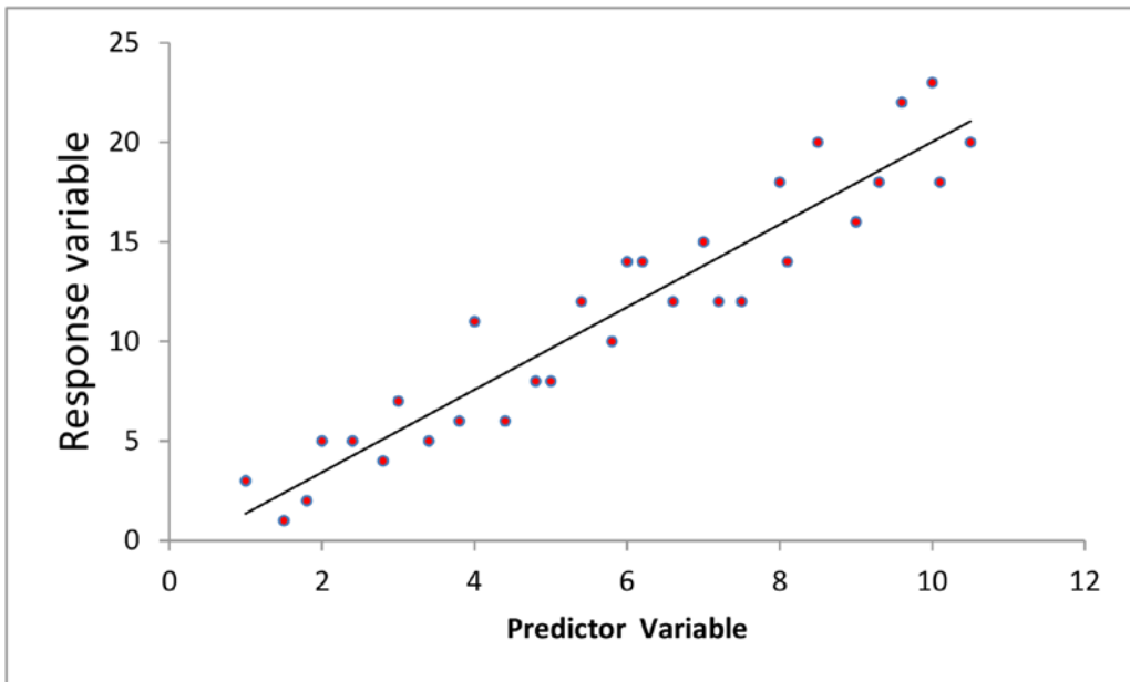
Figure 8-1. Linear regression
