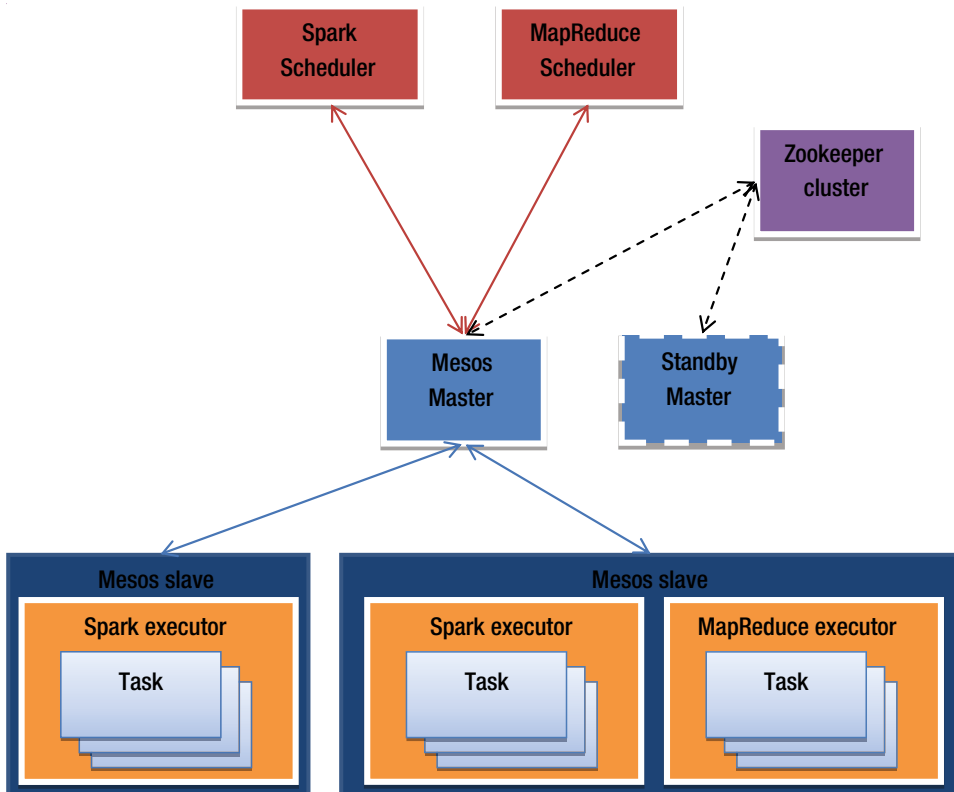
Figure 10-2. Mesos architecture
