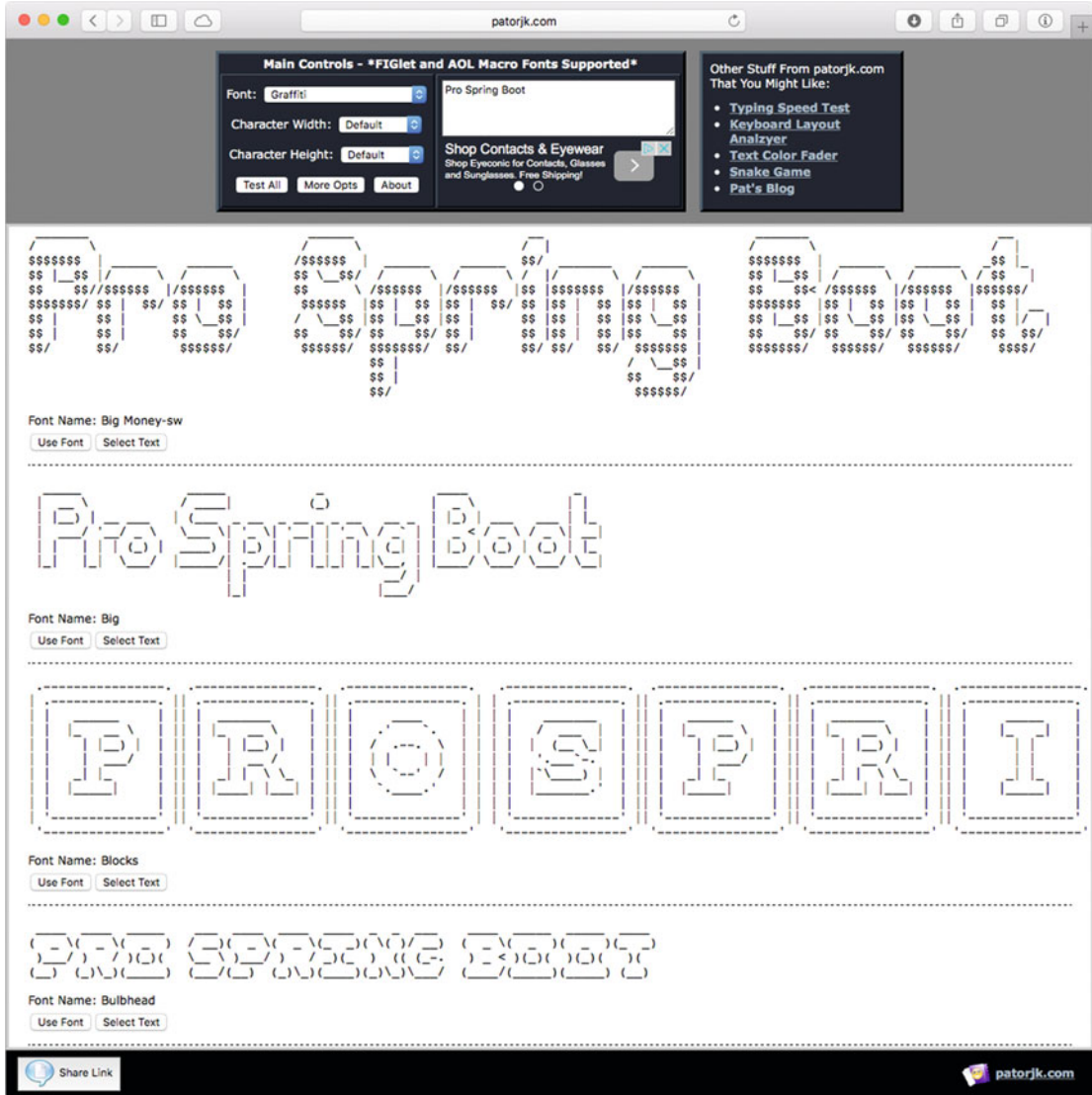
Figure 3-3. ASCII art
